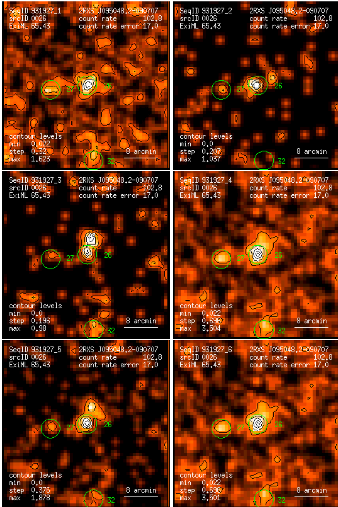
Figure 26: RASS 931927: detection 0026: band rate images, Gaussian filter: (1) PSPC channels 11 – 41, (2) 52 – 90, (3) 91 – 201, (4) 11 – 235, (5) 52 – 201, (6) 11 – 201. Broad band rates in counts/ks. Band rate contour levels in counts/ks/arcmin 2 .
