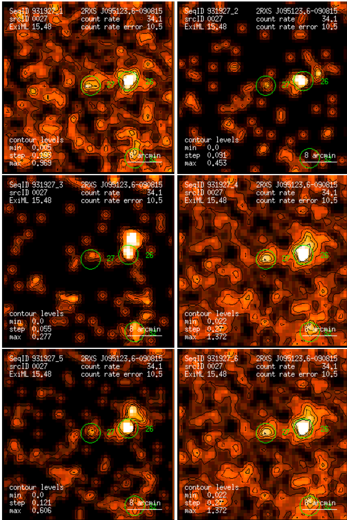
Figure 27: RASS 931927: detection 0027: band rate images, Gaussian filter: (1) PSPC channels 11 – 41, (2) 52 – 90, (3) 91 – 201, (4) 11 – 235, (5) 52 – 201, (6) 11 – 201. Broad band rates in counts/ks. Band rate contour levels in counts/ks/arcmin 2 .
