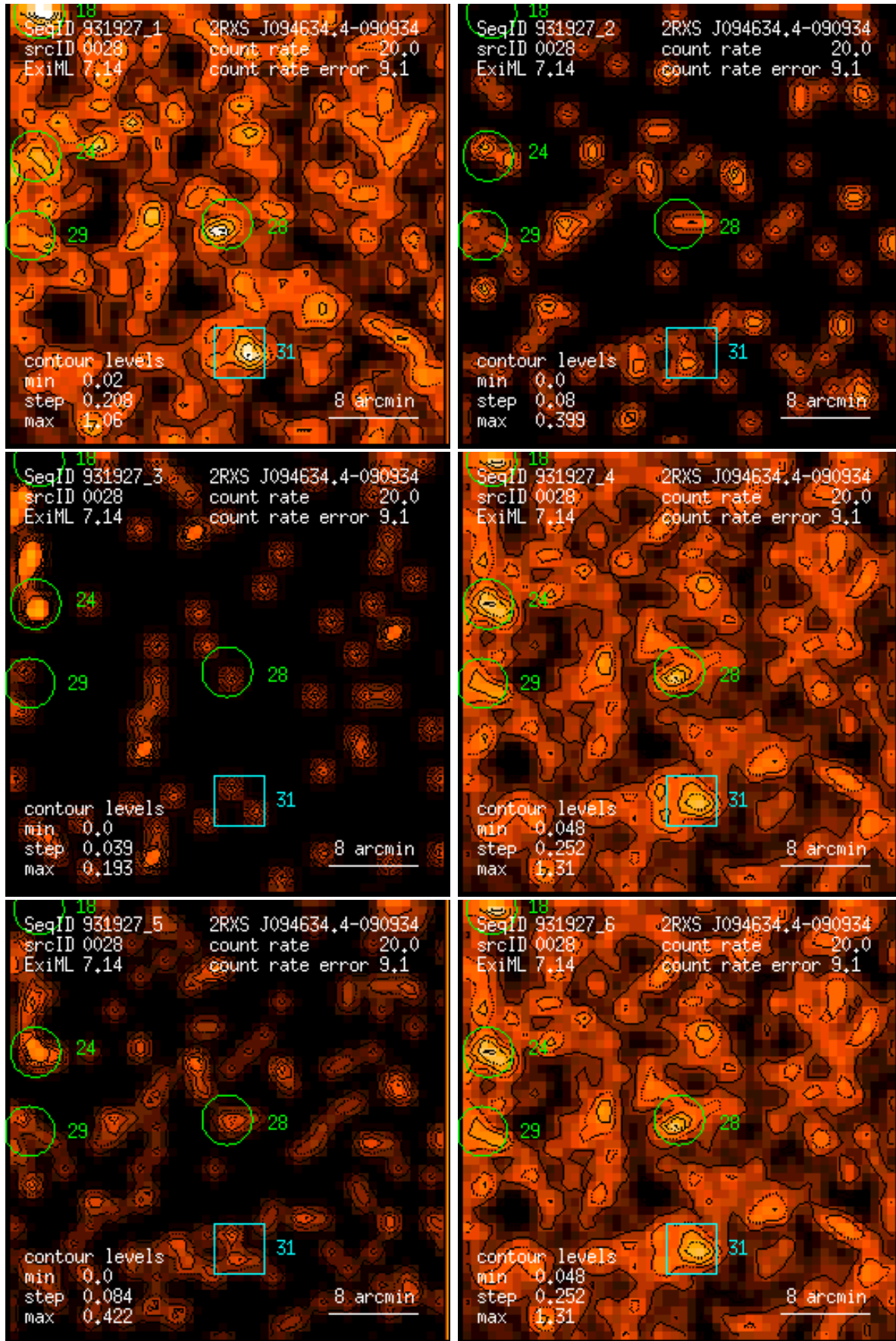
Figure 28: RASS 931927: detection 0028: band rate images, Gaussian filter: (1) PSPC channels 11 – 41, (2) 52 – 90, (3) 91 – 201, (4) 11 – 235, (5) 52 – 201, (6) 11 – 201. Broad band rates in counts/ks. Band rate contour levels in counts/ks/arcmin 2 .
