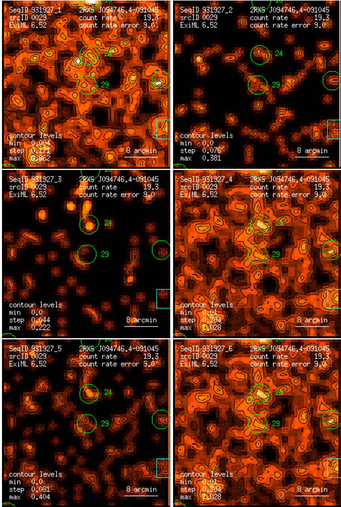
Figure 29: RASS 931927: detection 0029: band rate images, Gaussian filter: (1) PSPC channels 11 – 41, (2) 52 – 90, (3) 91 – 201, (4) 11 – 235, (5) 52 – 201, (6) 11 – 201. Broad band rates in counts/ks. Band rate contour levels in counts/ks/arcmin 2 .
