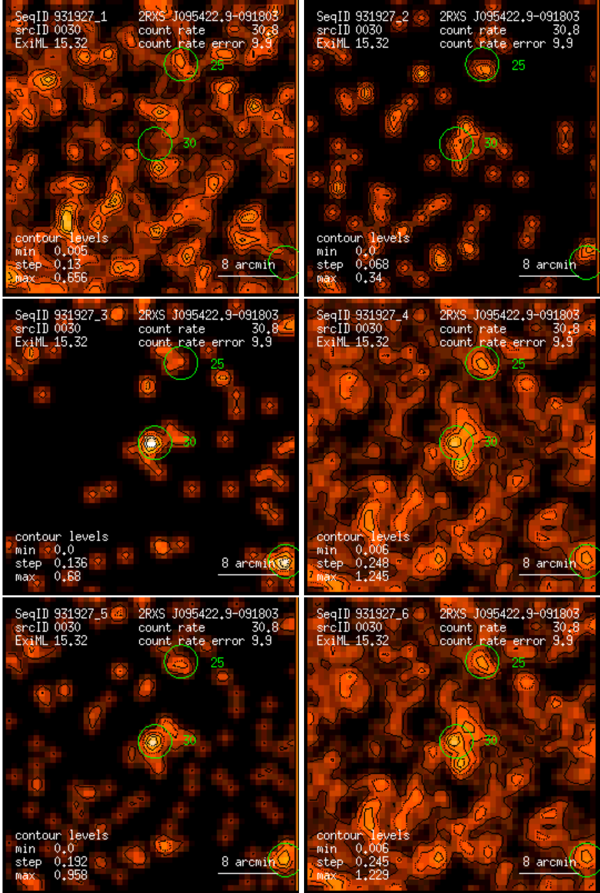
Figure 30: RASS 931927: detection 0030: band rate images, Gaussian filter: (1) PSPC channels 11 – 41, (2) 52 – 90, (3) 91 – 201, (4) 11 – 235, (5) 52 – 201, (6) 11 – 201. Broad band rates in counts/ks. Band rate contour levels in counts/ks/arcmin 2 .
