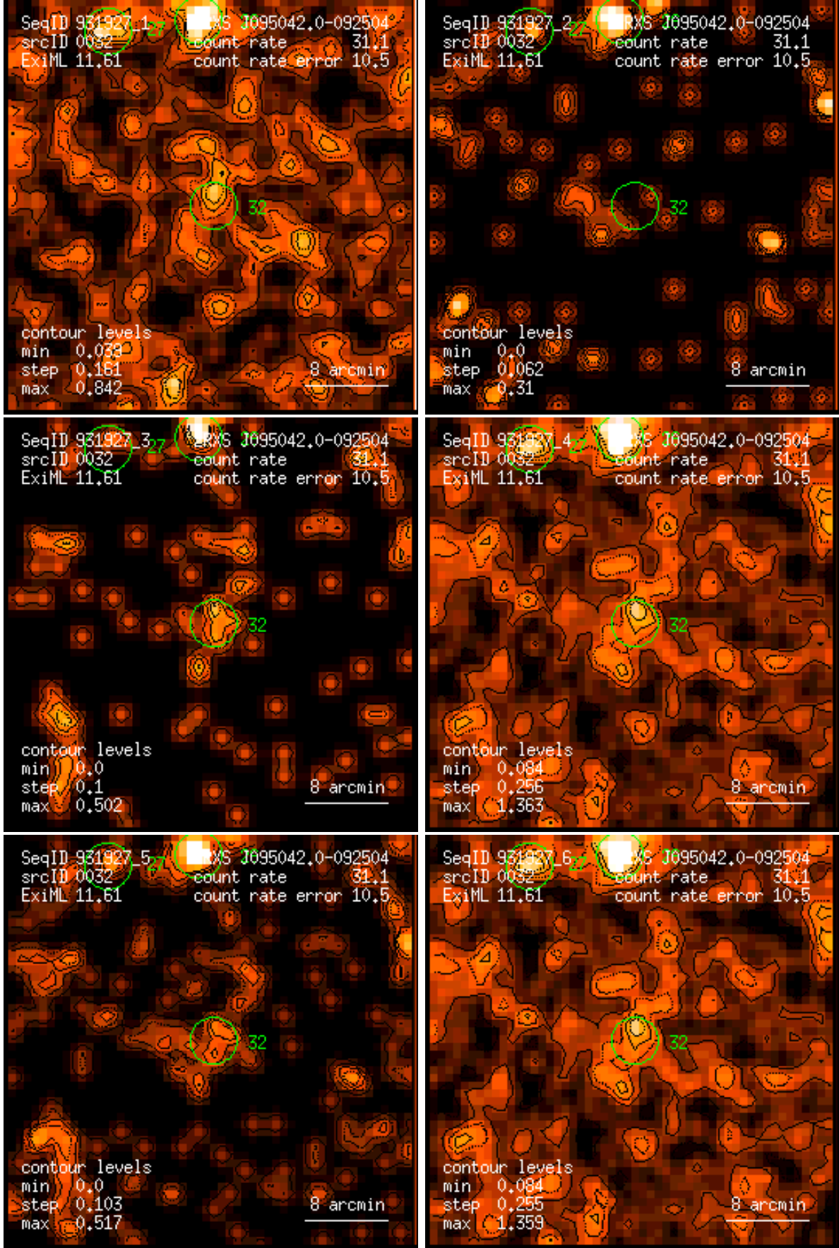
Figure 32: RASS 931927: detection 0032: band rate images, Gaussian filter: (1) PSPC channels 11 – 41, (2) 52 – 90, (3) 91 – 201, (4) 11 – 235, (5) 52 – 201, (6) 11 – 201. Broad band rates in counts/ks. Band rate contour levels in counts/ks/arcmin 2 .
