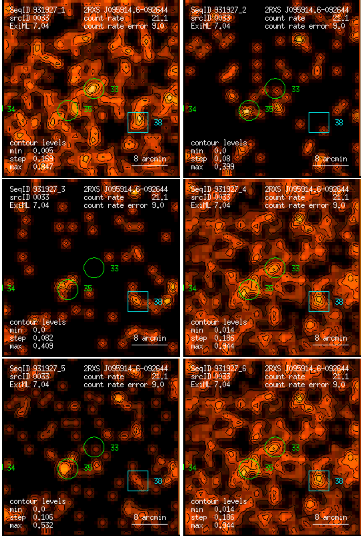
Figure 33: RASS 931927: detection 0033: band rate images, Gaussian filter: (1) PSPC channels 11 – 41, (2) 52 – 90, (3) 91 – 201, (4) 11 – 235, (5) 52 – 201, (6) 11 – 201. Broad band rates in counts/ks. Band rate contour levels in counts/ks/arcmin 2 .
