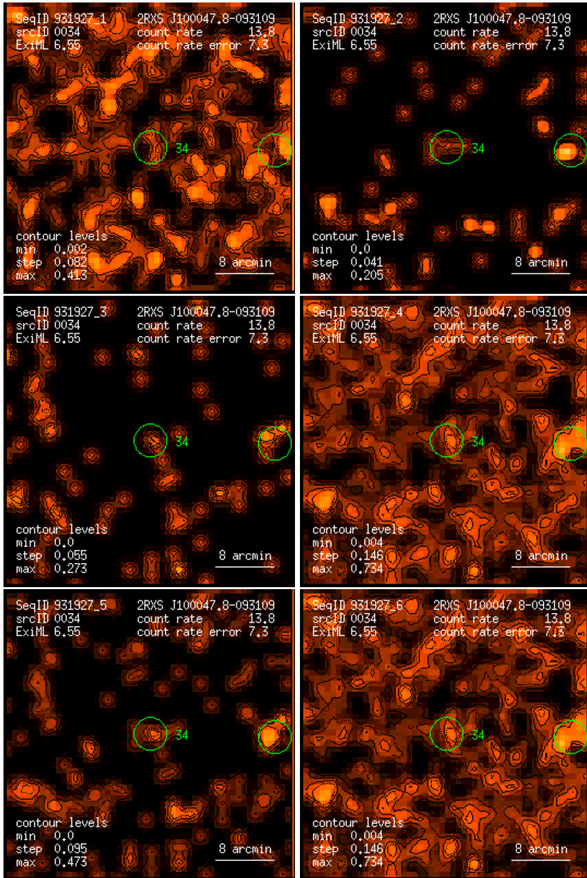
Figure 34: RASS 931927: detection 0034: band rate images, Gaussian filter: (1) PSPC channels 11 – 41, (2) 52 – 90, (3) 91 – 201, (4) 11 – 235, (5) 52 – 201, (6) 11 – 201. Broad band rates in counts/ks. Band rate contour levels in counts/ks/arcmin 2 .
