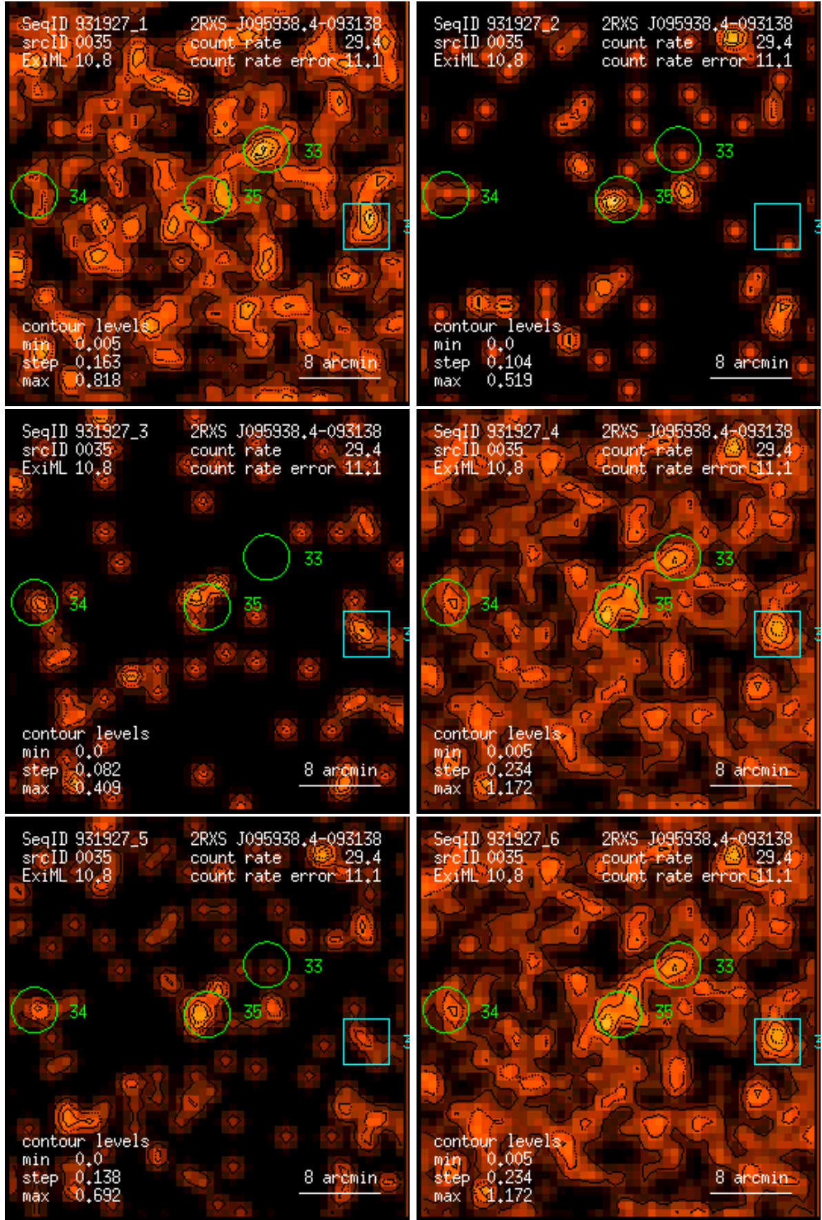
Figure 35: RASS 931927: detection 0035: band rate images, Gaussian filter: (1) PSPC channels 11 – 41, (2) 52 – 90, (3) 91 – 201, (4) 11 – 235, (5) 52 – 201, (6) 11 – 201. Broad band rates in counts/ks. Band rate contour levels in counts/ks/arcmin 2 .
