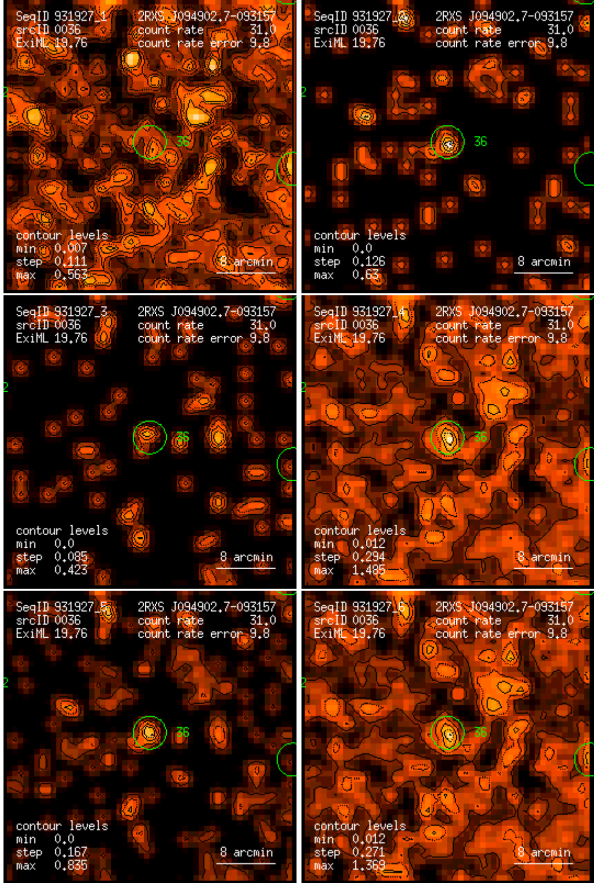
Figure 36: RASS 931927: detection 0036: band rate images, Gaussian filter: (1) PSPC channels 11 – 41, (2) 52 – 90, (3) 91 – 201, (4) 11 – 235, (5) 52 – 201, (6) 11 – 201. Broad band rates in counts/ks. Band rate contour levels in counts/ks/arcmin 2 .
