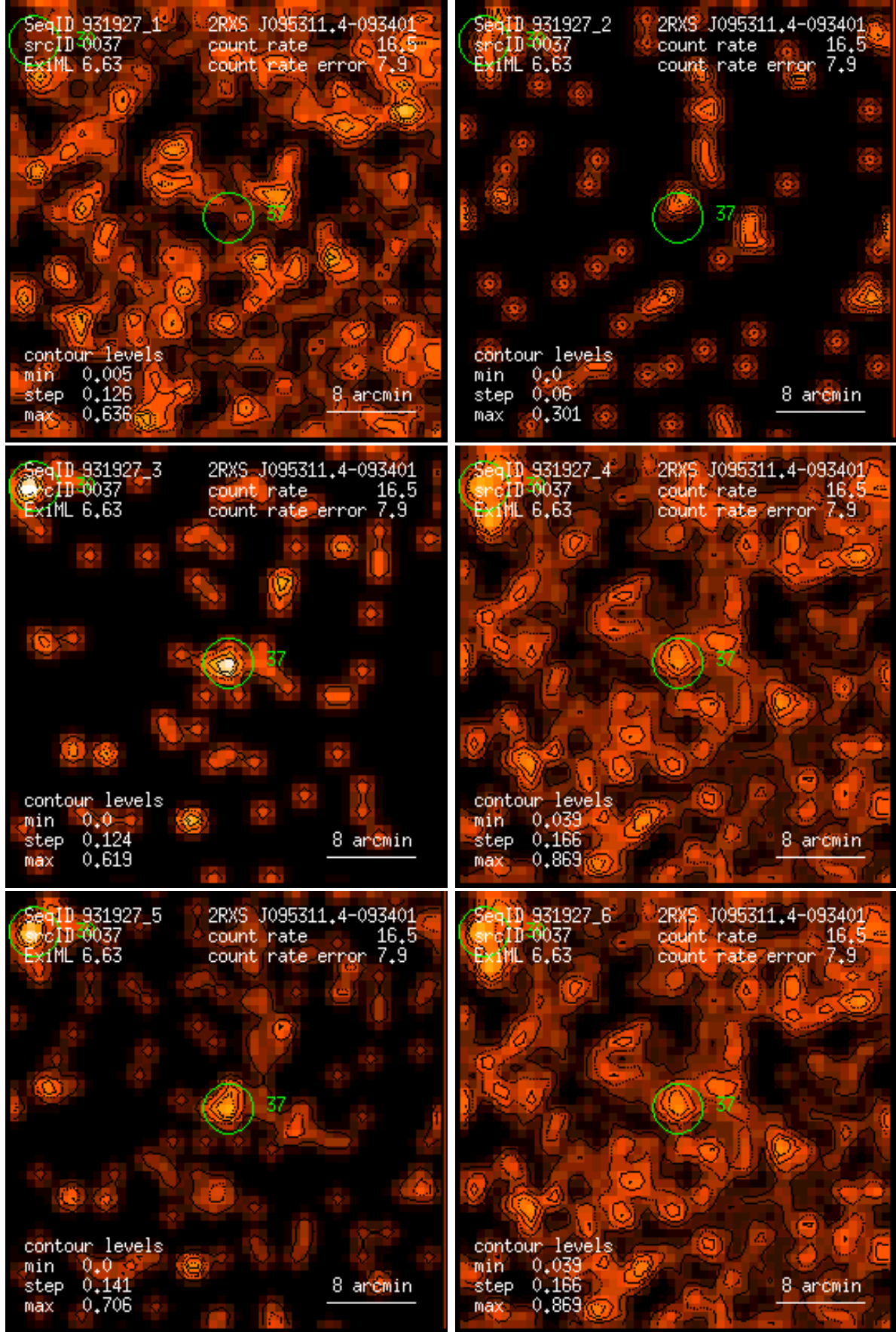
Figure 37: RASS 931927: detection 0037: band rate images, Gaussian filter: (1) PSPC channels 11 – 41, (2) 52 – 90, (3) 91 – 201, (4) 11 – 235, (5) 52 – 201, (6) 11 – 201. Broad band rates in counts/ks. Band rate contour levels in counts/ks/arcmin 2 .
