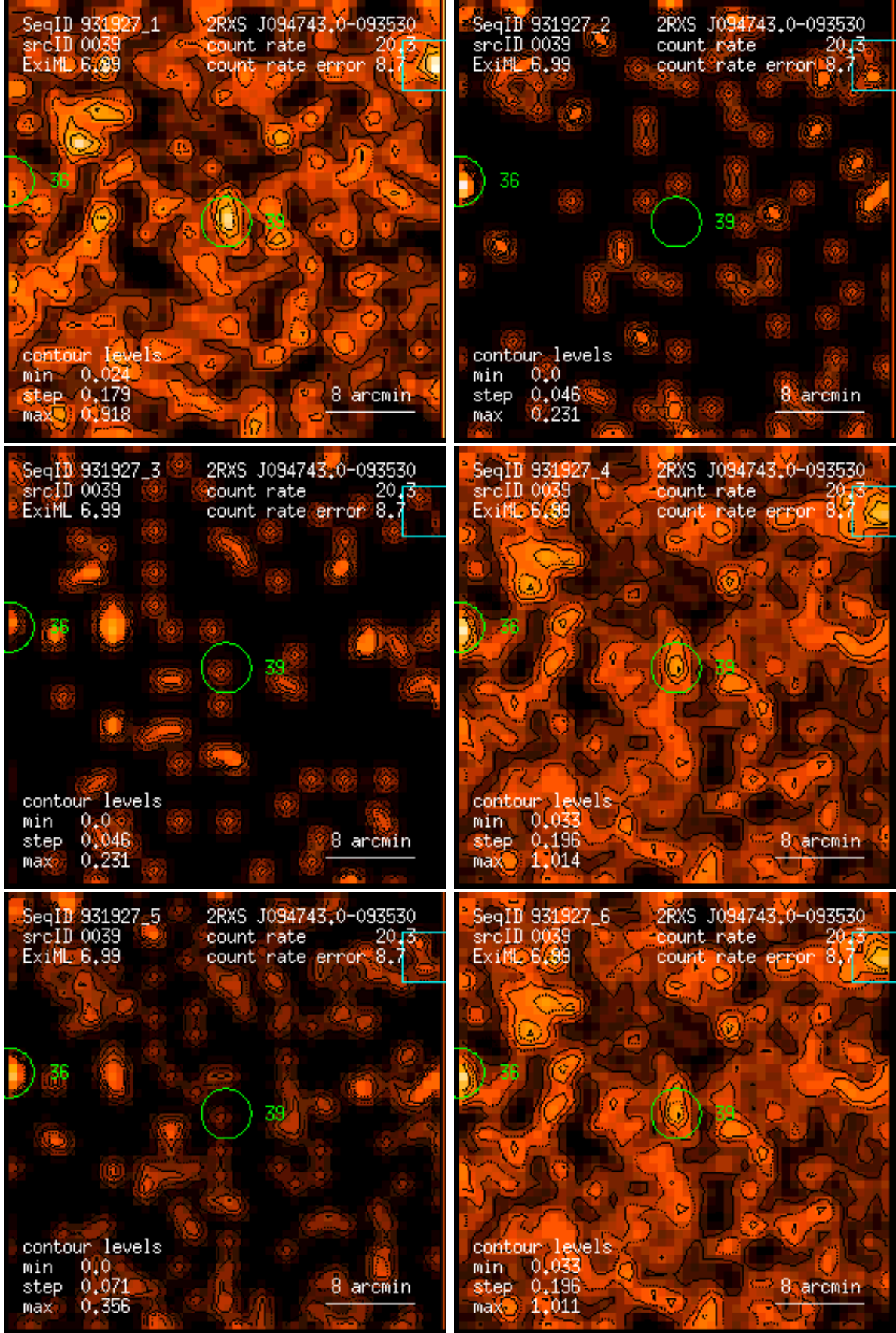
Figure 39: RASS 931927: detection 0039: band rate images, Gaussian filter: (1) PSPC channels 11 – 41, (2) 52 – 90, (3) 91 – 201, (4) 11 – 235, (5) 52 – 201, (6) 11 – 201. Broad band rates in counts/ks. Band rate contour levels in counts/ks/arcmin 2 .
