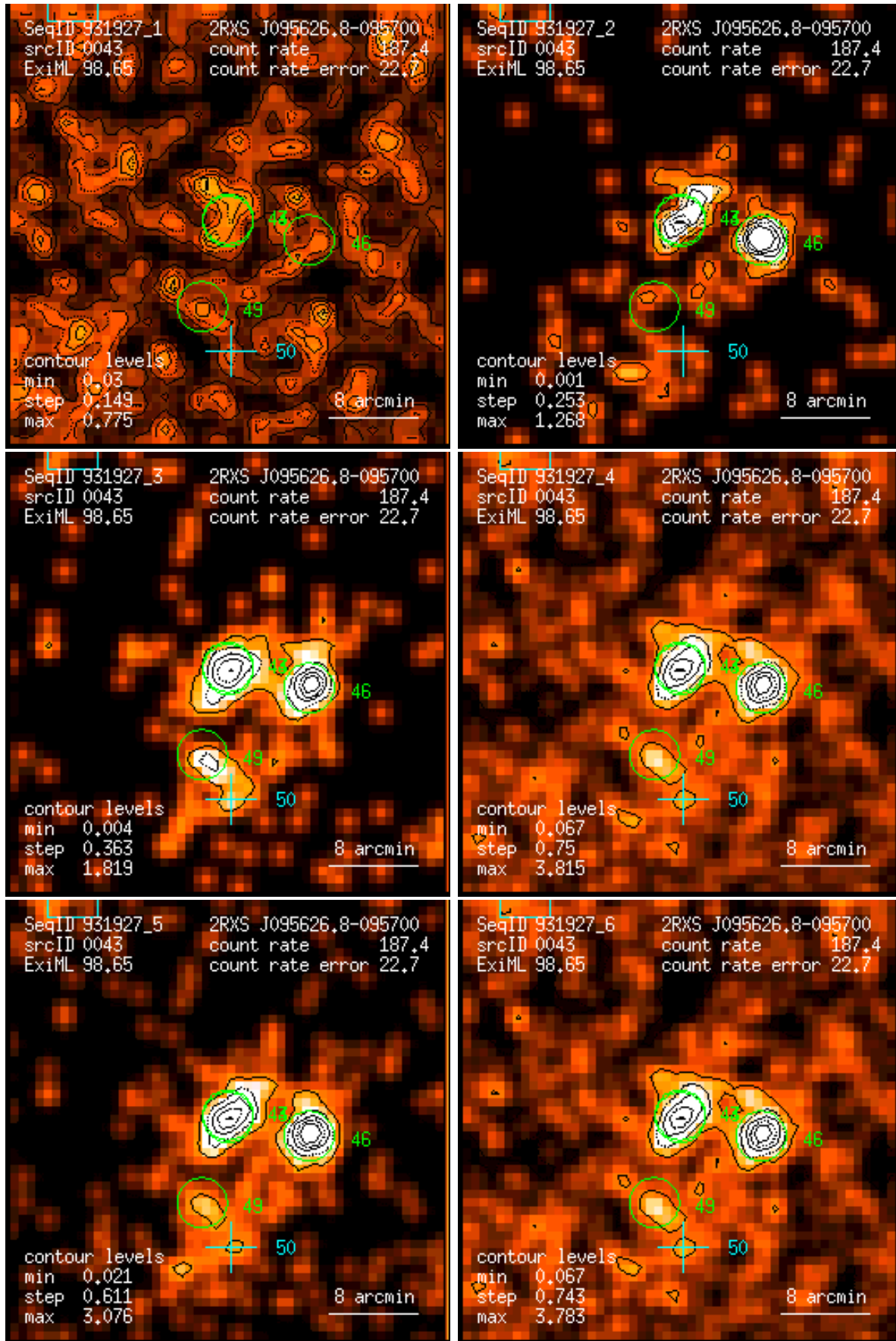
Figure 43: RASS 931927: detection 0043: band rate images, Gaussian filter: (1) PSPC channels 11 – 41, (2) 52 – 90, (3) 91 – 201, (4) 11 – 235, (5) 52 – 201, (6) 11 – 201. Broad band rates in counts/ks. Band rate contour levels in counts/ks/arcmin 2 .
