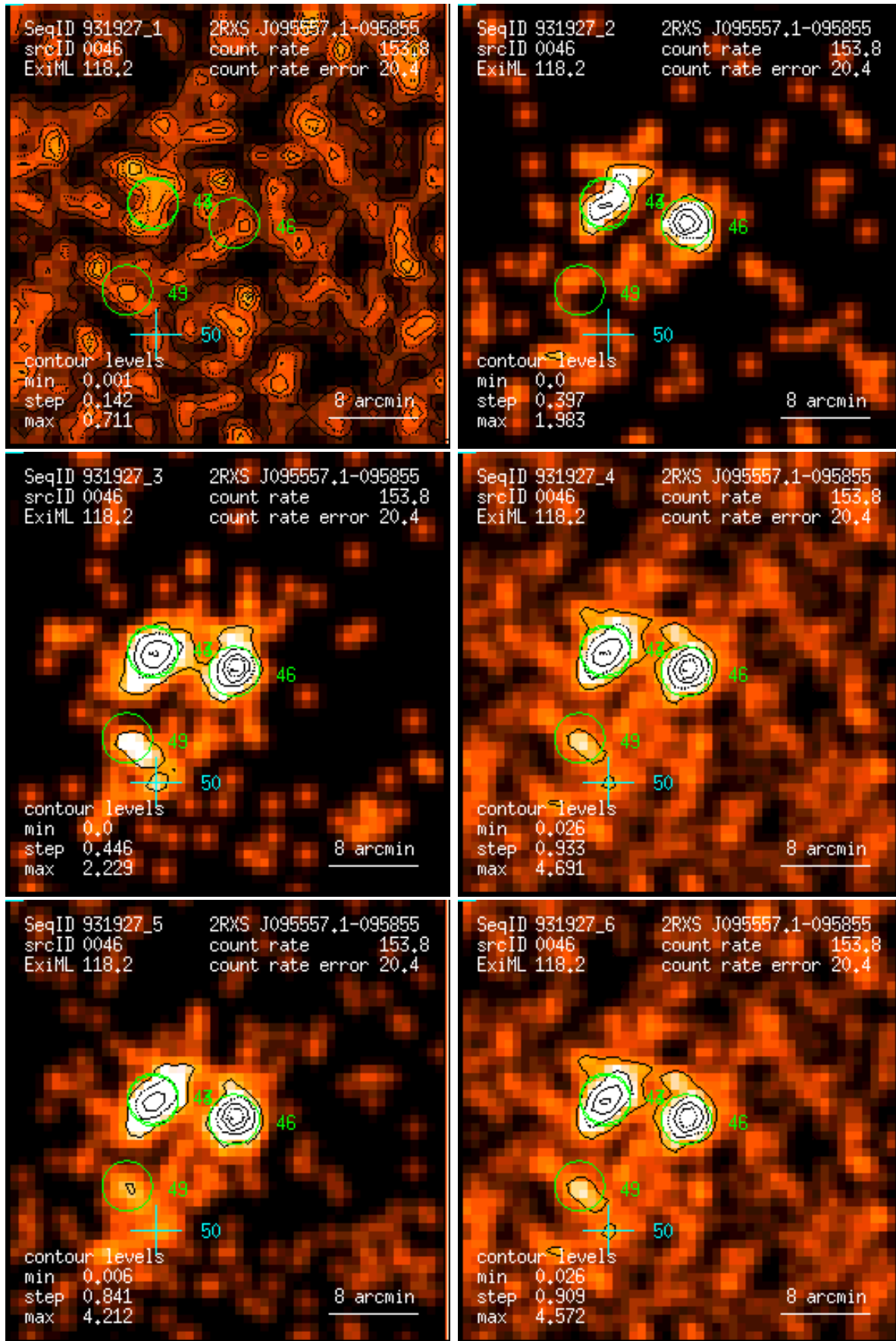
Figure 46: RASS 931927: detection 0046: band rate images, Gaussian filter: (1) PSPC channels 11 – 41, (2) 52 – 90, (3) 91 – 201, (4) 11 – 235, (5) 52 – 201, (6) 11 – 201. Broad band rates in counts/ks. Band rate contour levels in counts/ks/arcmin 2 .
