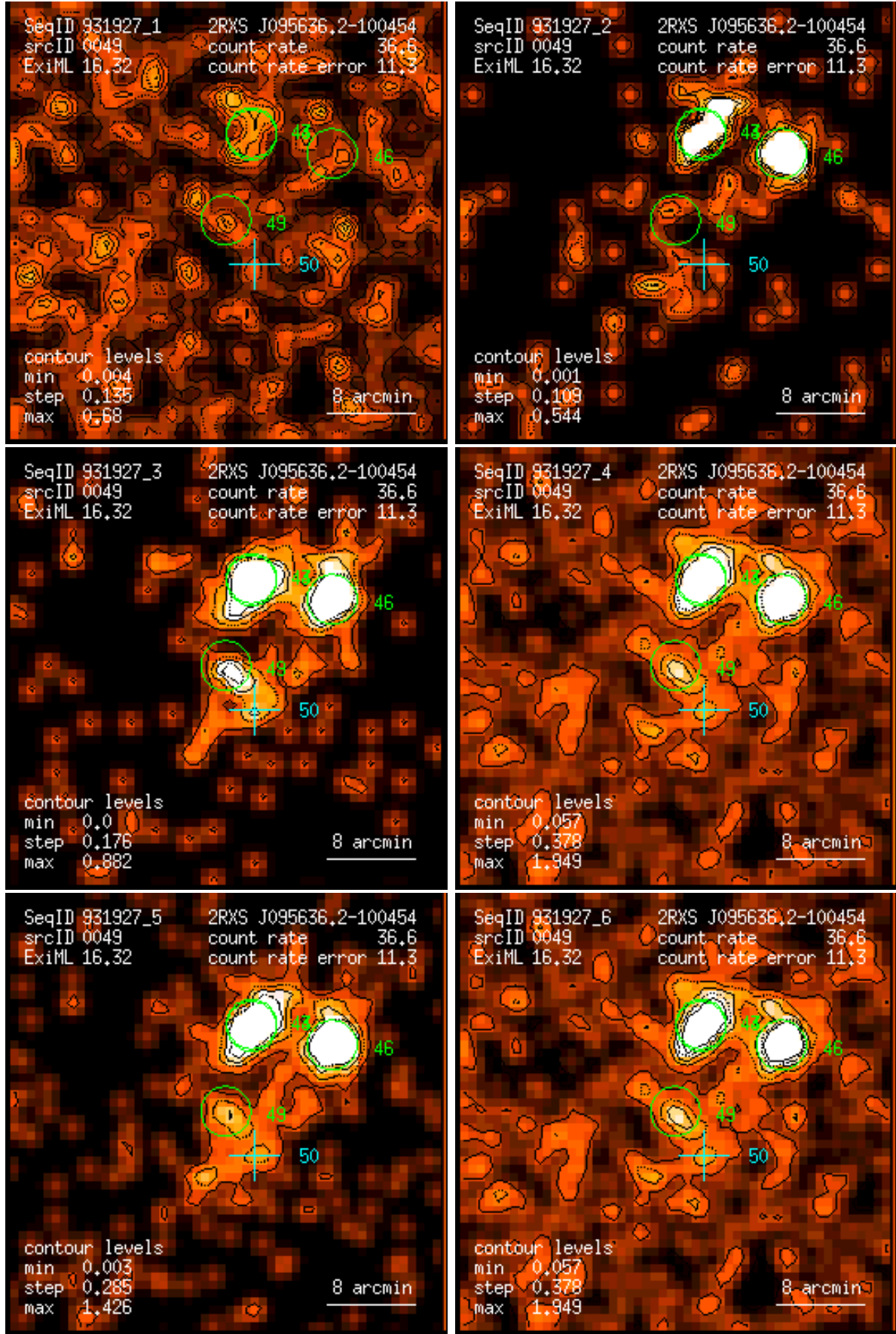
Figure 49: RASS 931927: detection 0049: band rate images, Gaussian filter: (1) PSPC channels 11 – 41, (2) 52 – 90, (3) 91 – 201, (4) 11 – 235, (5) 52 – 201, (6) 11 – 201. Broad band rates in counts/ks. Band rate contour levels in counts/ks/arcmin 2 .
