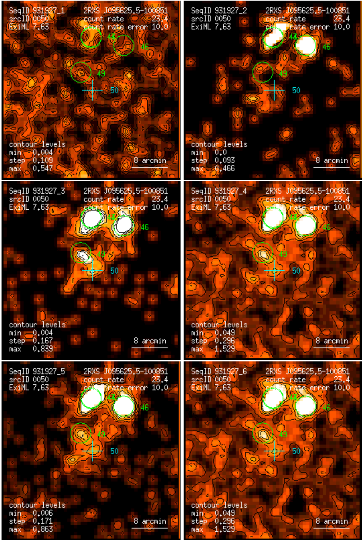
Figure 50: RASS 931927: detection 0050: band rate images, Gaussian filter: (1) PSPC channels 11 – 41, (2) 52 – 90, (3) 91 – 201, (4) 11 – 235, (5) 52 – 201, (6) 11 – 201. Broad band rates in counts/ks. Band rate contour levels in counts/ks/arcmin 2 .
