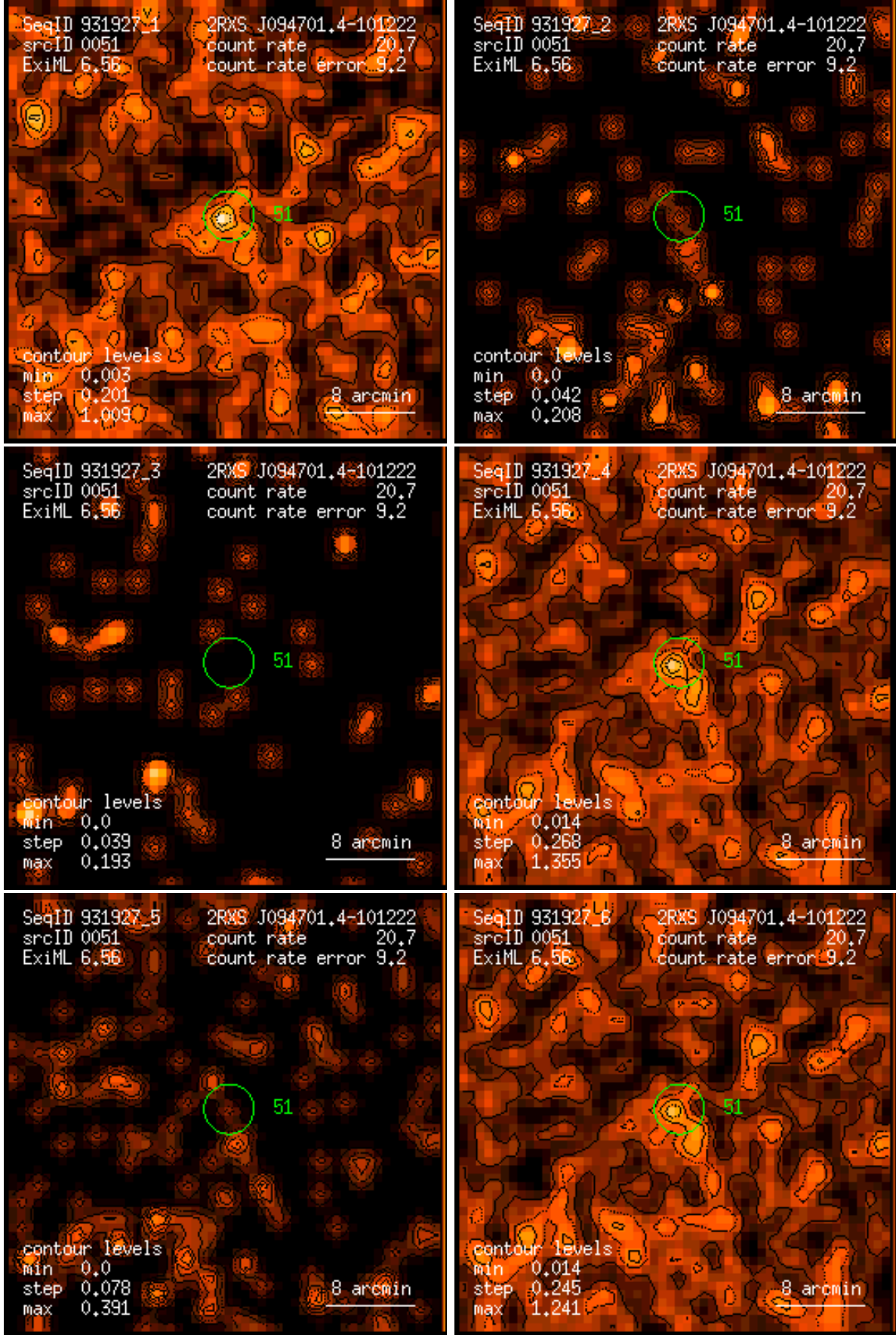
Figure 51: RASS 931927: detection 0051: band rate images, Gaussian filter: (1) PSPC channels 11 – 41, (2) 52 – 90, (3) 91 – 201, (4) 11 – 235, (5) 52 – 201, (6) 11 – 201. Broad band rates in counts/ks. Band rate contour levels in counts/ks/arcmin 2 .
