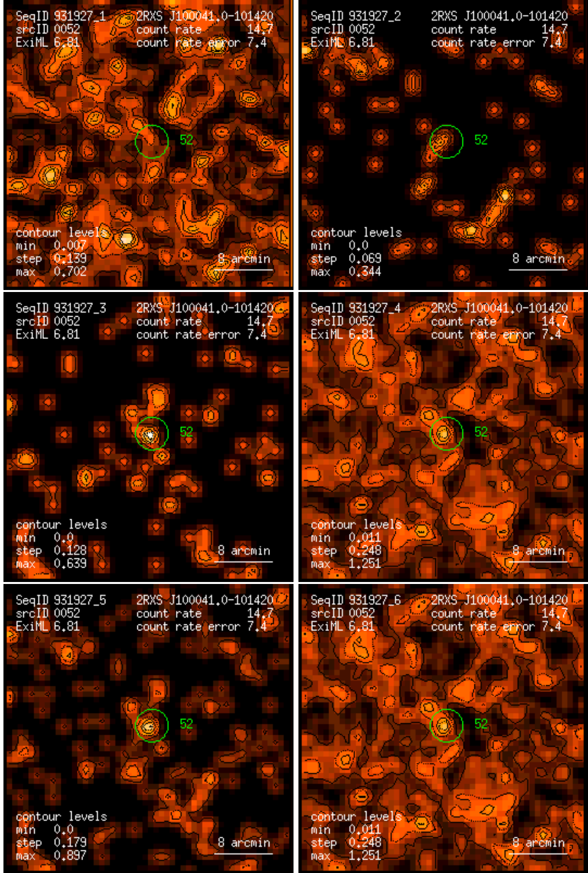
Figure 52: RASS 931927: detection 0052: band rate images, Gaussian filter: (1) PSPC channels 11 – 41, (2) 52 – 90, (3) 91 – 201, (4) 11 – 235, (5) 52 – 201, (6) 11 – 201. Broad band rates in counts/ks. Band rate contour levels in counts/ks/arcmin 2 .
