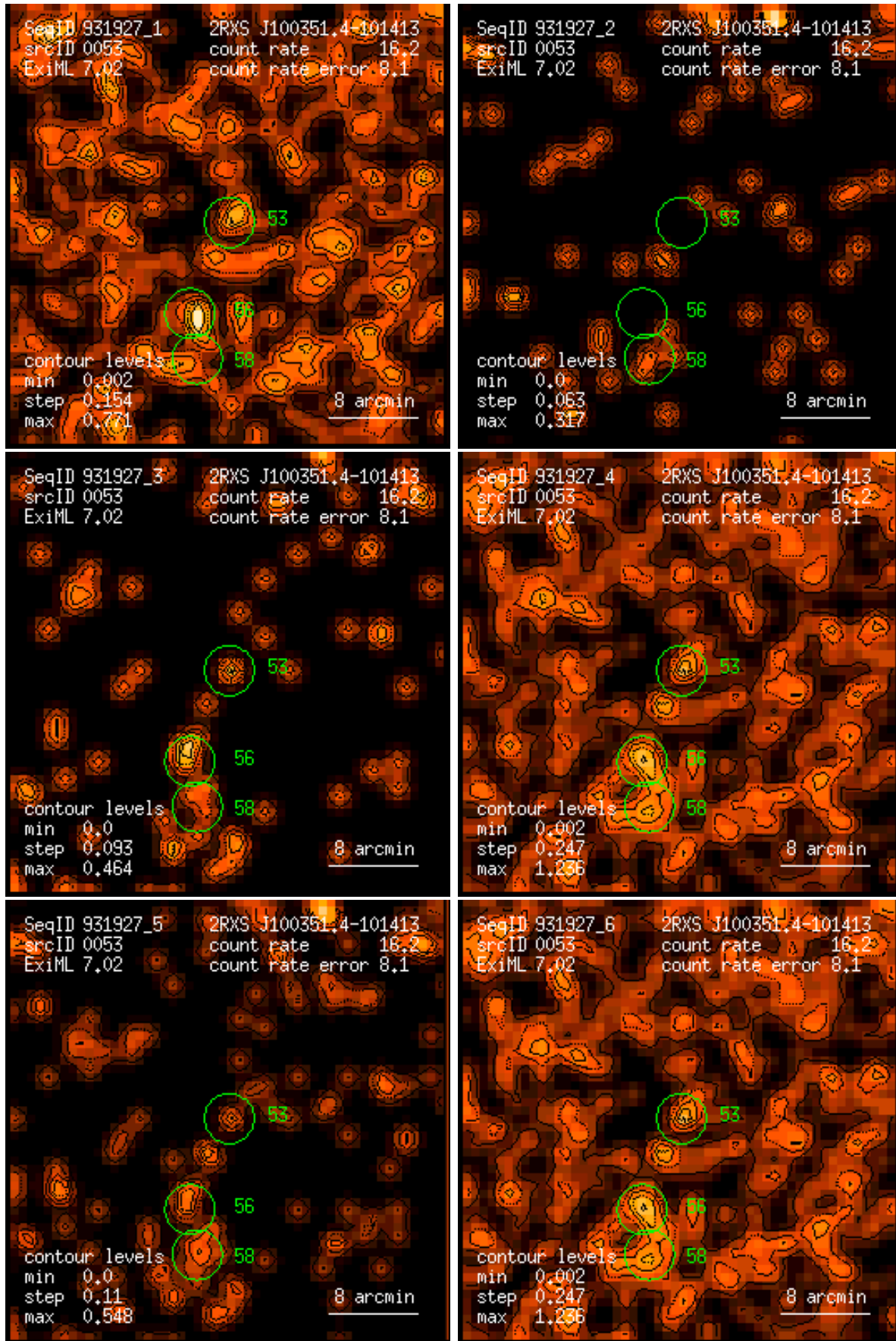
Figure 53: RASS 931927: detection 0053: band rate images, Gaussian filter: (1) PSPC channels 11 – 41, (2) 52 – 90, (3) 91 – 201, (4) 11 – 235, (5) 52 – 201, (6) 11 – 201. Broad band rates in counts/ks. Band rate contour levels in counts/ks/arcmin 2 .
