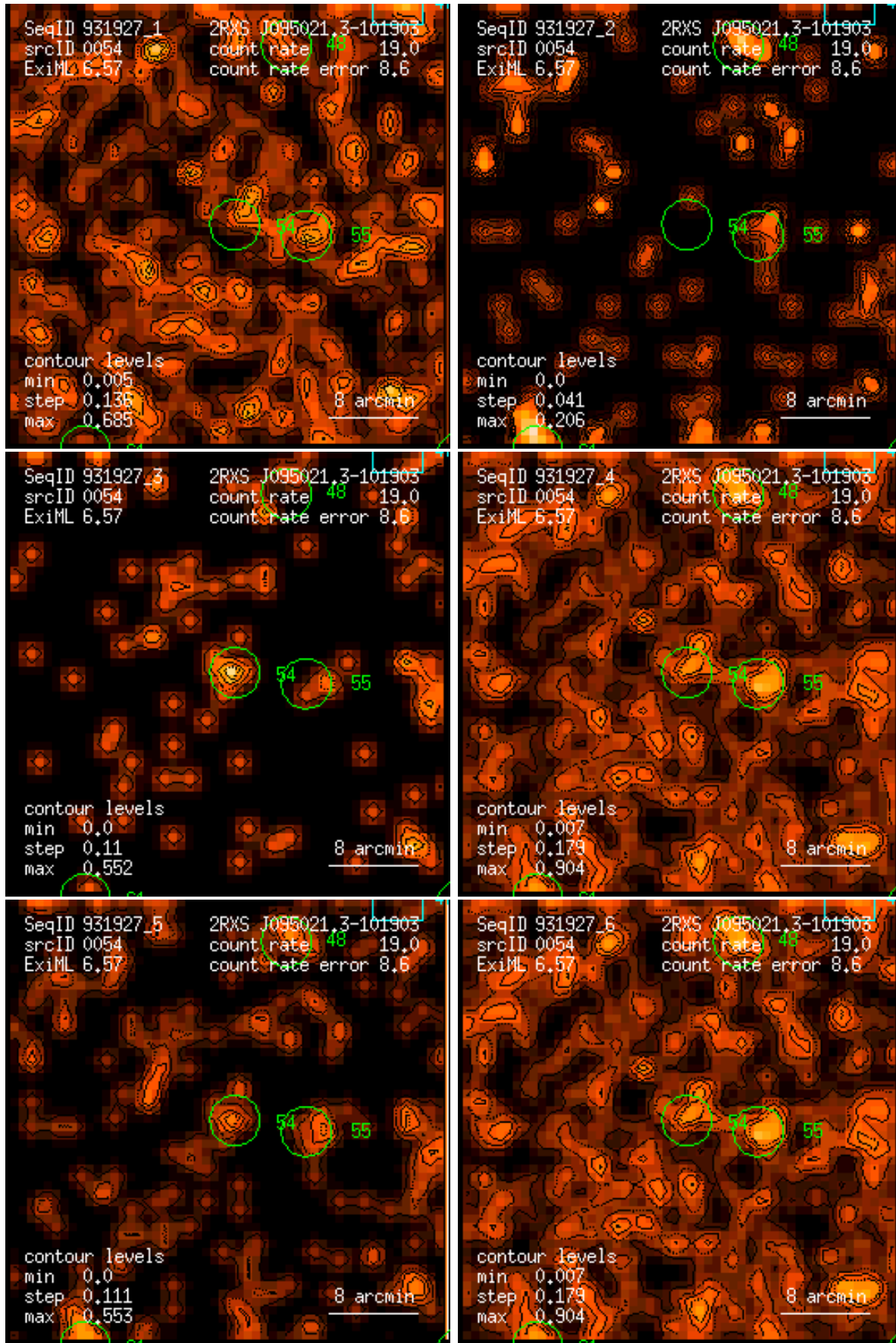
Figure 54: RASS 931927: detection 0054: band rate images, Gaussian filter: (1) PSPC channels 11 – 41, (2) 52 – 90, (3) 91 – 201, (4) 11 – 235, (5) 52 – 201, (6) 11 – 201. Broad band rates in counts/ks. Band rate contour levels in counts/ks/arcmin 2 .
