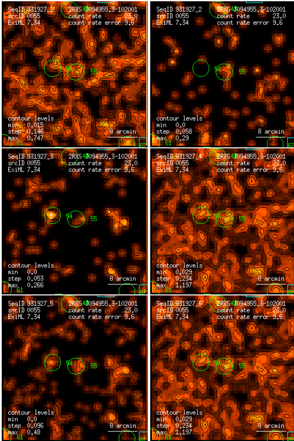
Figure 55: RASS 931927: detection 0055: band rate images, Gaussian filter: (1) PSPC channels 11 – 41, (2) 52 – 90, (3) 91 – 201, (4) 11 – 235, (5) 52 – 201, (6) 11 – 201. Broad band rates in counts/ks. Band rate contour levels in counts/ks/arcmin 2 .
