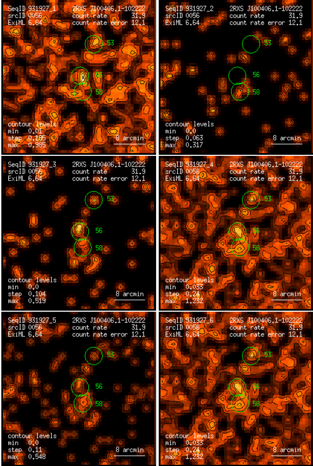
Figure 56: RASS 931927: detection 0056: band rate images, Gaussian filter: (1) PSPC channels 11 – 41, (2) 52 – 90, (3) 91 – 201, (4) 11 – 235, (5) 52 – 201, (6) 11 – 201. Broad band rates in counts/ks. Band rate contour levels in counts/ks/arcmin 2 .
