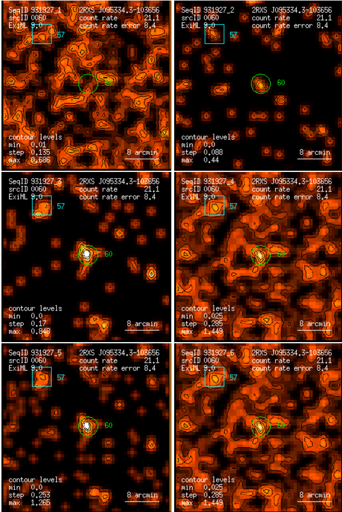
Figure 60: RASS 931927: detection 0060: band rate images, Gaussian filter: (1) PSPC channels 11 – 41, (2) 52 – 90, (3) 91 – 201, (4) 11 – 235, (5) 52 – 201, (6) 11 – 201. Broad band rates in counts/ks. Band rate contour levels in counts/ks/arcmin 2 .
