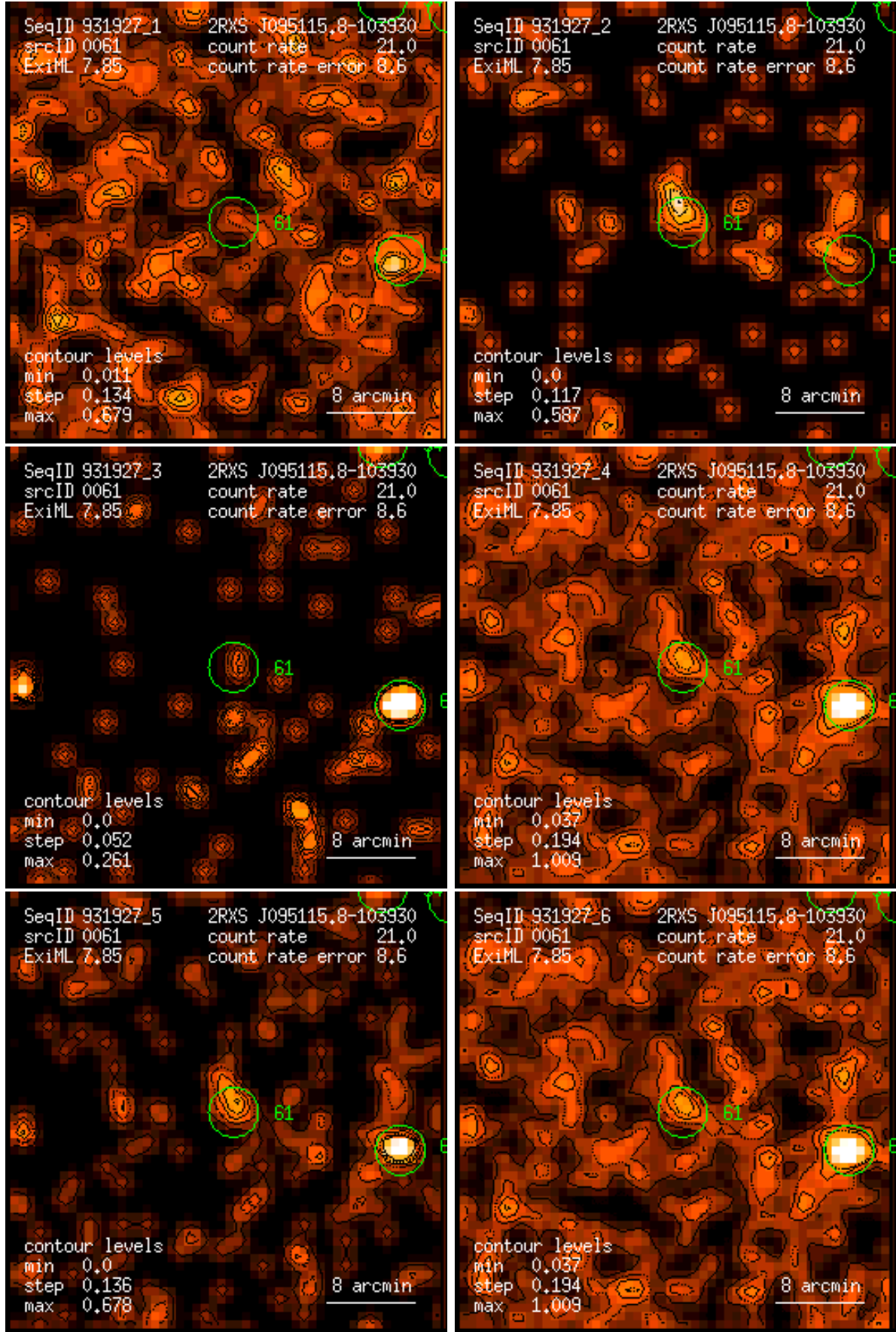
Figure 61: RASS 931927: detection 0061: band rate images, Gaussian filter: (1) PSPC channels 11 – 41, (2) 52 – 90, (3) 91 – 201, (4) 11 – 235, (5) 52 – 201, (6) 11 – 201. Broad band rates in counts/ks. Band rate contour levels in counts/ks/arcmin 2 .
