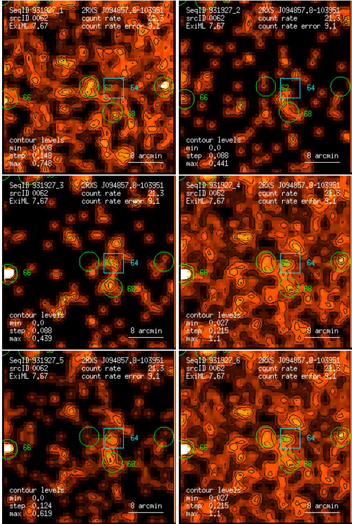
Figure 62: RASS 931927: detection 0062: band rate images, Gaussian filter: (1) PSPC channels 11 – 41, (2) 52 – 90, (3) 91 – 201, (4) 11 – 235, (5) 52 – 201, (6) 11 – 201. Broad band rates in counts/ks. Band rate contour levels in counts/ks/arcmin 2 .
