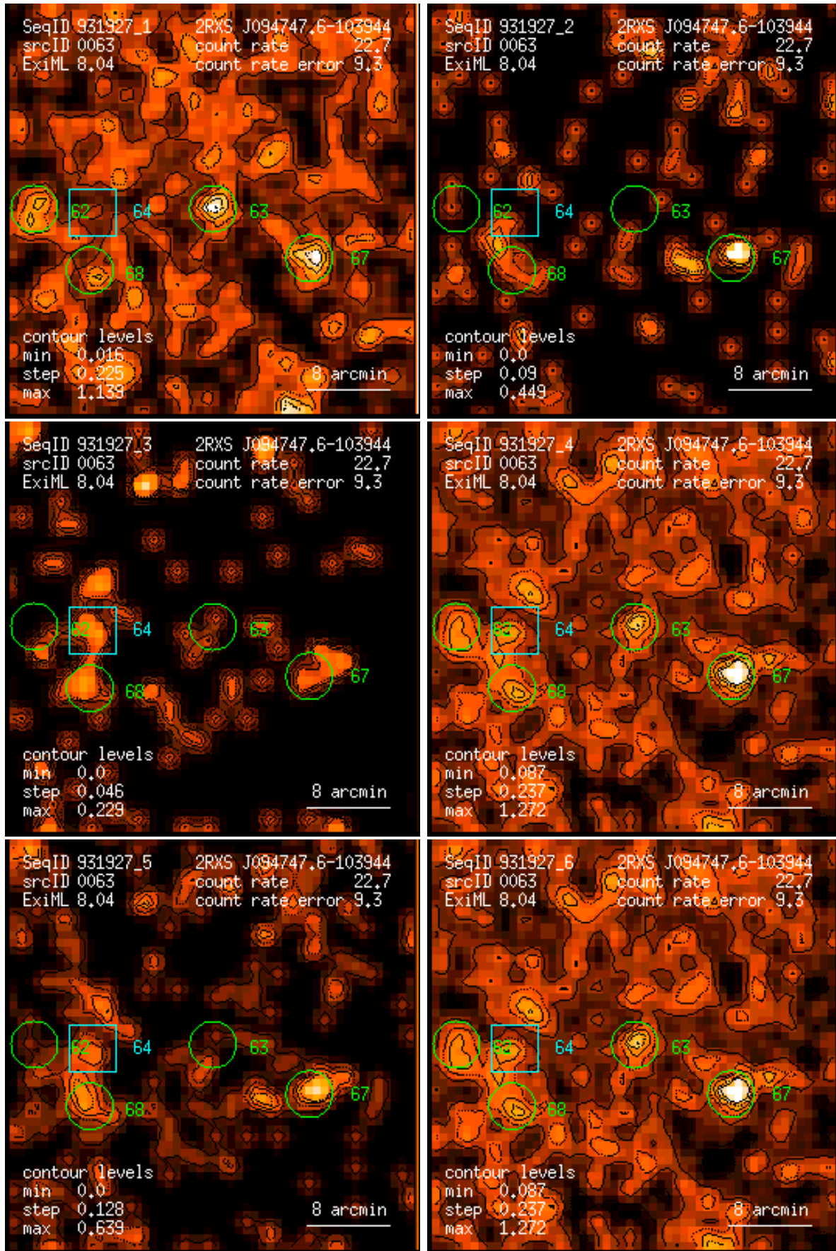
Figure 63: RASS 931927: detection 0063: band rate images, Gaussian filter: (1) PSPC channels 11 – 41, (2) 52 – 90, (3) 91 – 201, (4) 11 – 235, (5) 52 – 201, (6) 11 – 201. Broad band rates in counts/ks. Band rate contour levels in counts/ks/arcmin 2 .
