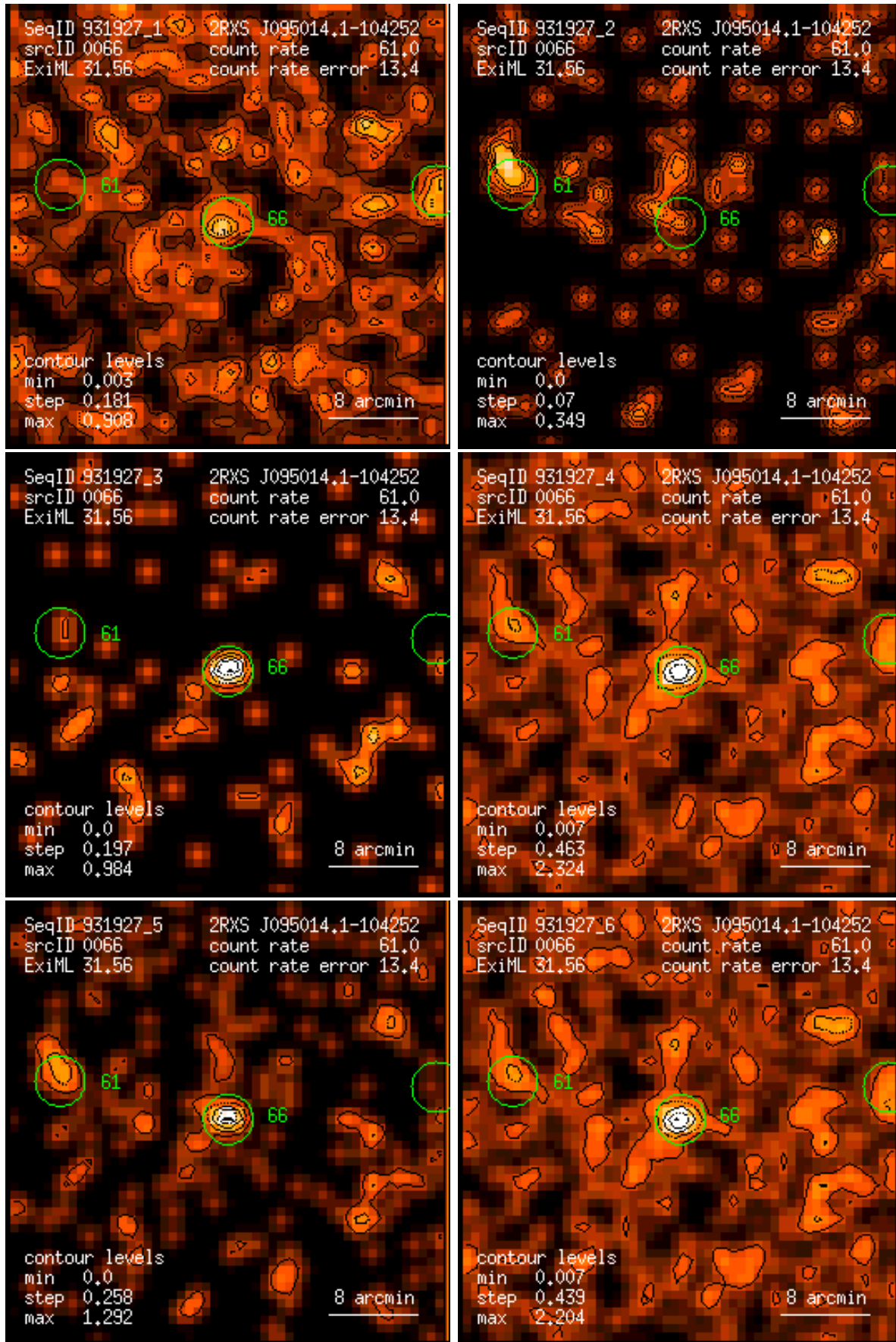
Figure 66: RASS 931927: detection 0066: band rate images, Gaussian filter: (1) PSPC channels 11 – 41, (2) 52 – 90, (3) 91 – 201, (4) 11 – 235, (5) 52 – 201, (6) 11 – 201. Broad band rates in counts/ks. Band rate contour levels in counts/ks/arcmin 2 .
