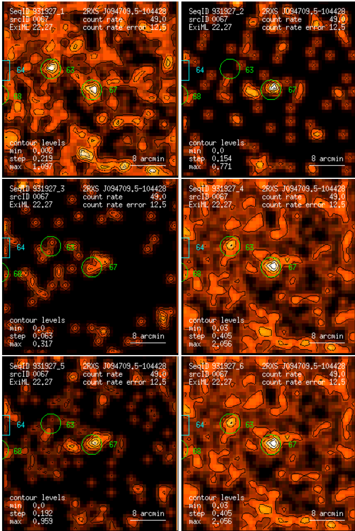
Figure 67: RASS 931927: detection 0067: band rate images, Gaussian filter: (1) PSPC channels 11 – 41, (2) 52 – 90, (3) 91 – 201, (4) 11 – 235, (5) 52 – 201, (6) 11 – 201. Broad band rates in counts/ks. Band rate contour levels in counts/ks/arcmin 2 .
