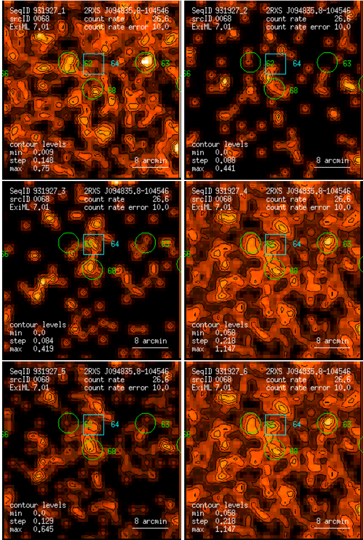
Figure 68: RASS 931927: detection 0068: band rate images, Gaussian filter: (1) PSPC channels 11 – 41, (2) 52 – 90, (3) 91 – 201, (4) 11 – 235, (5) 52 – 201, (6) 11 – 201. Broad band rates in counts/ks. Band rate contour levels in counts/ks/arcmin 2 .
