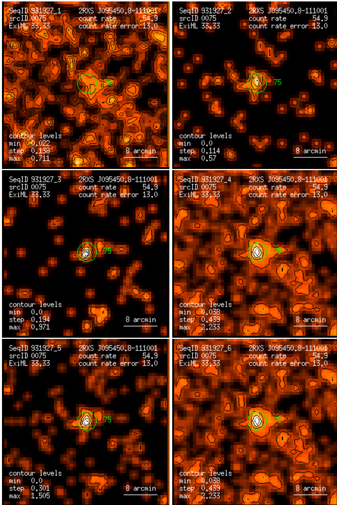
Figure 75: RASS 931927: detection 0075: band rate images, Gaussian filter: (1) PSPC channels 11 – 41, (2) 52 – 90, (3) 91 – 201, (4) 11 – 235, (5) 52 – 201, (6) 11 – 201. Broad band rates in counts/ks. Band rate contour levels in counts/ks/arcmin 2 .
