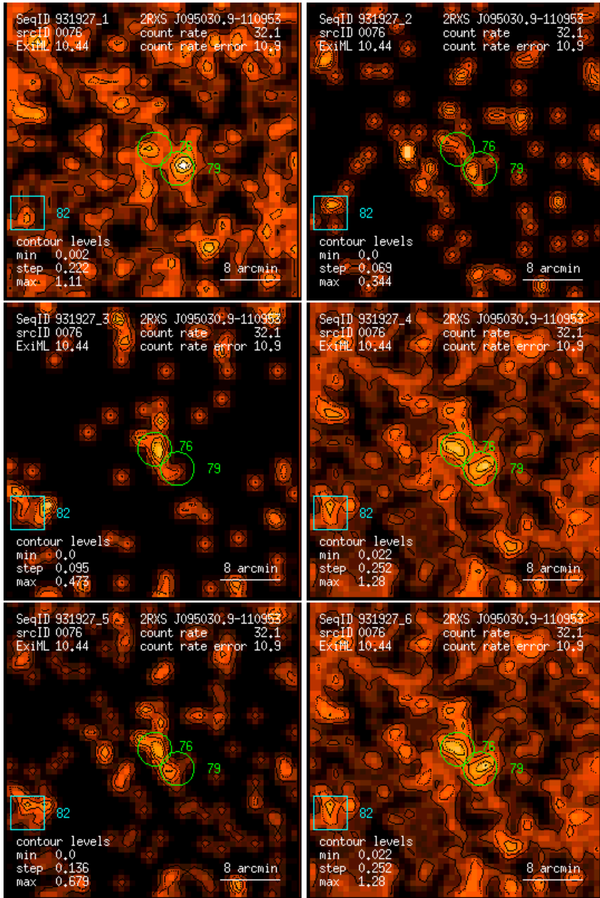
Figure 76: RASS 931927: detection 0076: band rate images, Gaussian filter: (1) PSPC channels 11 – 41, (2) 52 – 90, (3) 91 – 201, (4) 11 – 235, (5) 52 – 201, (6) 11 – 201. Broad band rates in counts/ks. Band rate contour levels in counts/ks/arcmin 2 .
