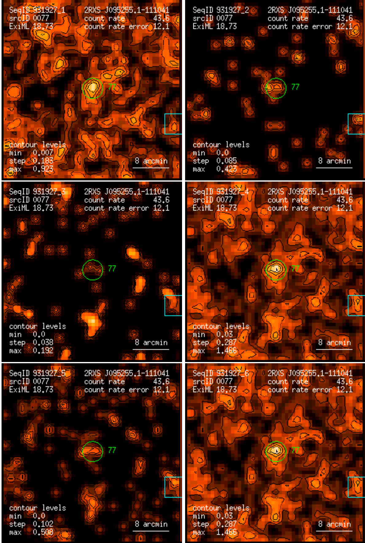
Figure 77: RASS 931927: detection 0077: band rate images, Gaussian filter: (1) PSPC channels 11 – 41, (2) 52 – 90, (3) 91 – 201, (4) 11 – 235, (5) 52 – 201, (6) 11 – 201. Broad band rates in counts/ks. Band rate contour levels in counts/ks/arcmin 2 .
