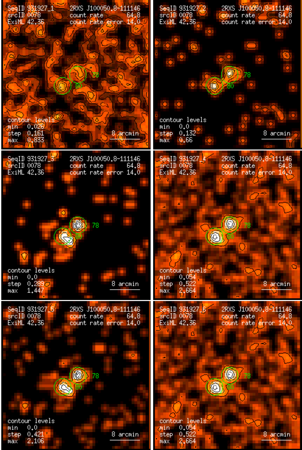
Figure 78: RASS 931927: detection 0078: band rate images, Gaussian filter: (1) PSPC channels 11 – 41, (2) 52 – 90, (3) 91 – 201, (4) 11 – 235, (5) 52 – 201, (6) 11 – 201. Broad band rates in counts/ks. Band rate contour levels in counts/ks/arcmin 2 .
