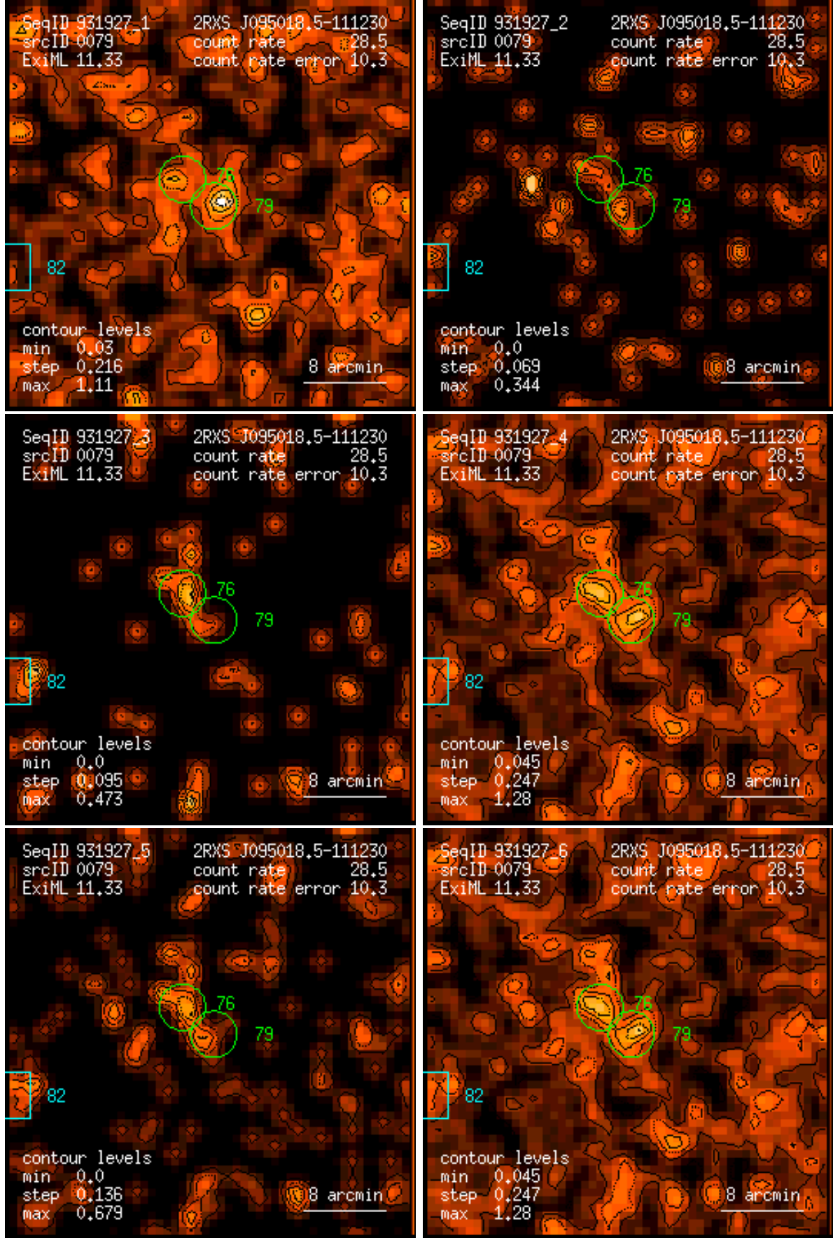
Figure 79: RASS 931927: detection 0079: band rate images, Gaussian filter: (1) PSPC channels 11 – 41, (2) 52 – 90, (3) 91 – 201, (4) 11 – 235, (5) 52 – 201, (6) 11 – 201. Broad band rates in counts/ks. Band rate contour levels in counts/ks/arcmin 2 .
