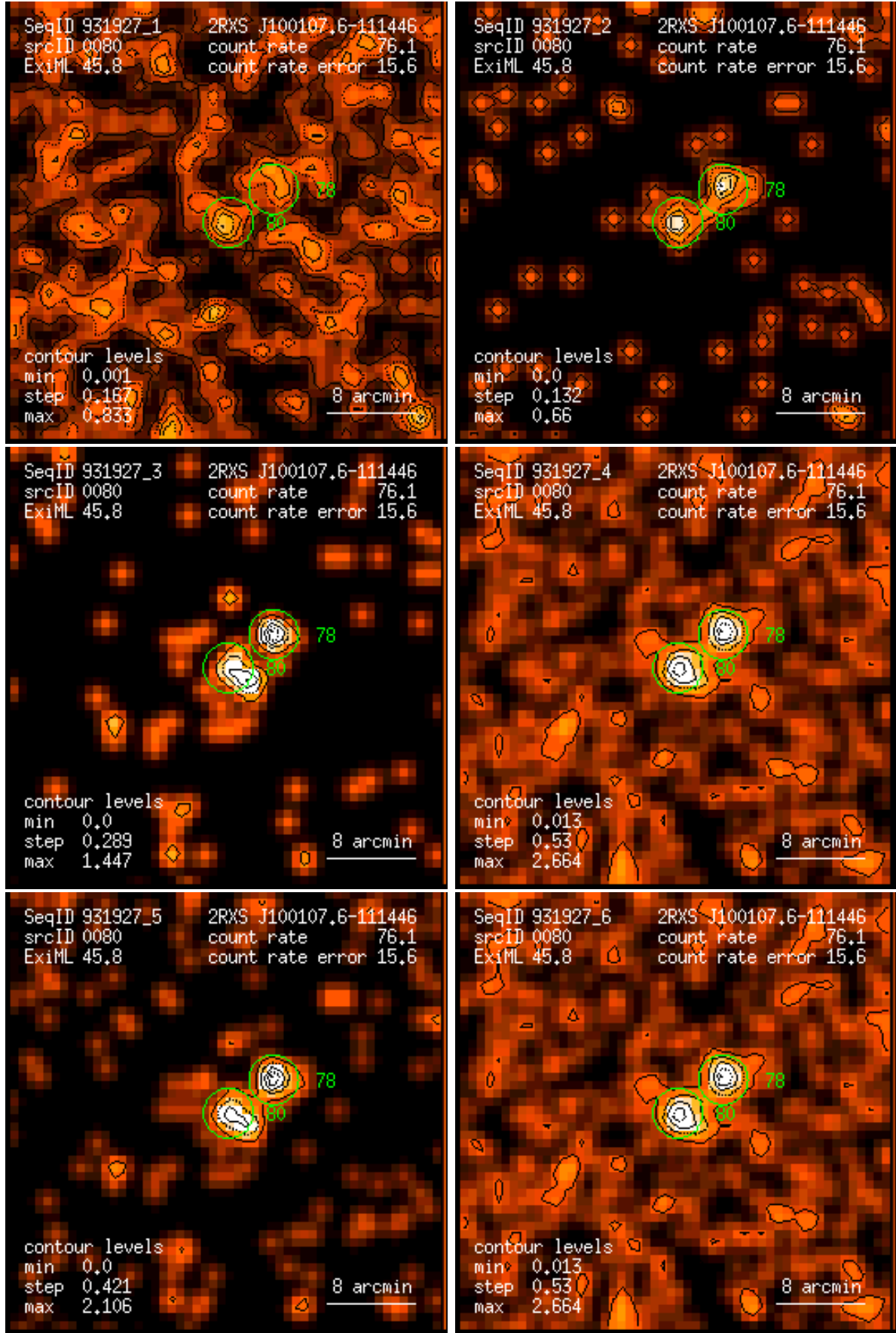
Figure 80: RASS 931927: detection 0080: band rate images, Gaussian filter: (1) PSPC channels 11 – 41, (2) 52 – 90, (3) 91 – 201, (4) 11 – 235, (5) 52 – 201, (6) 11 – 201. Broad band rates in counts/ks. Band rate contour levels in counts/ks/arcmin 2 .
