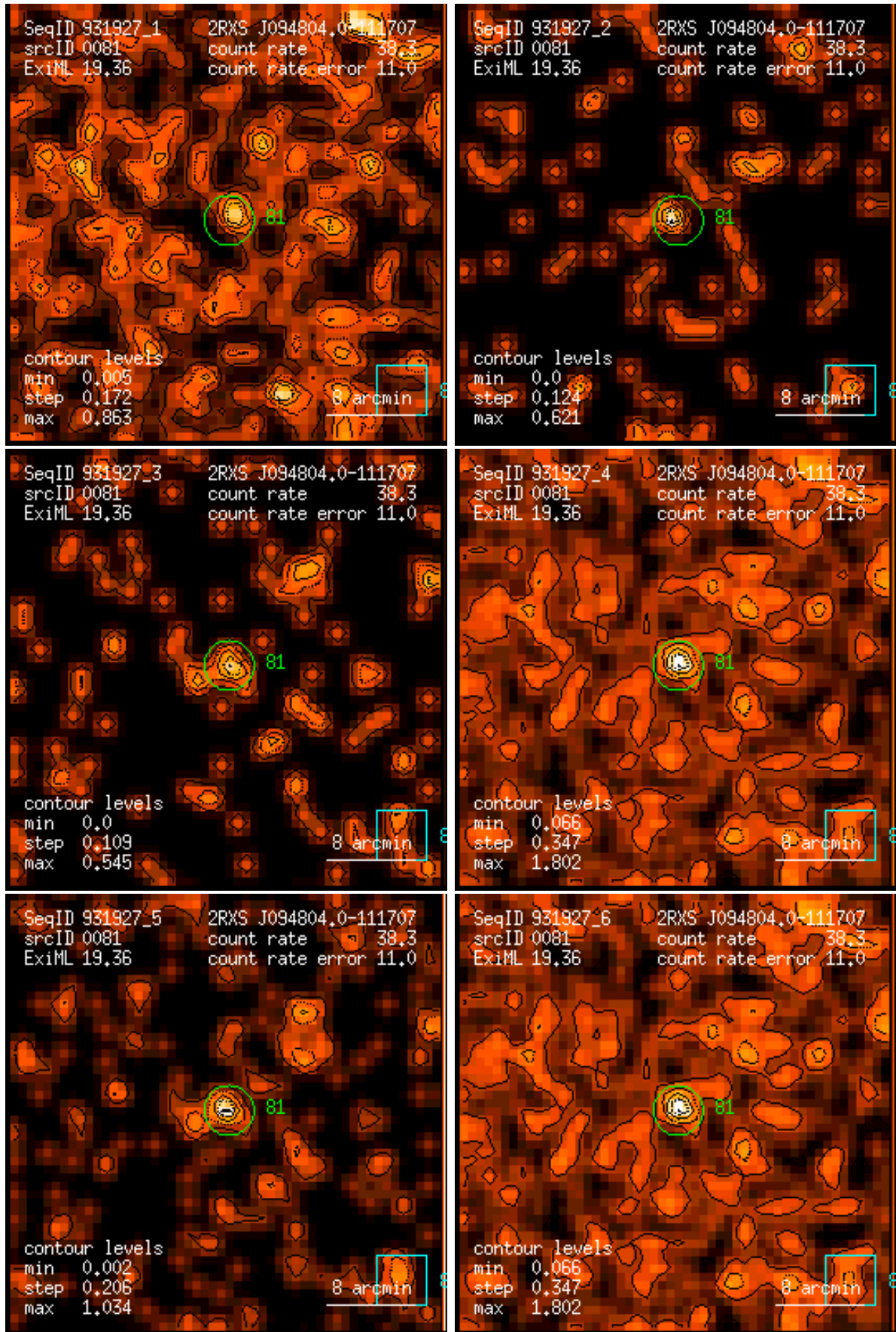
Figure 81: RASS 931927: detection 0081: band rate images, Gaussian filter: (1) PSPC channels 11 – 41, (2) 52 – 90, (3) 91 – 201, (4) 11 – 235, (5) 52 – 201, (6) 11 – 201. Broad band rates in counts/ks. Band rate contour levels in counts/ks/arcmin 2 .
