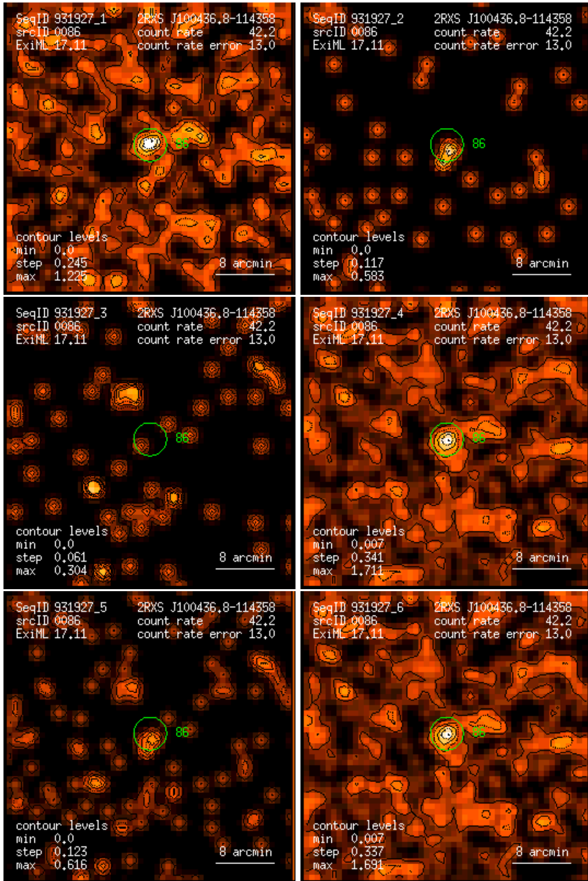
Figure 86: RASS 931927: detection 0086: band rate images, Gaussian filter: (1) PSPC channels 11 – 41, (2) 52 – 90, (3) 91 – 201, (4) 11 – 235, (5) 52 – 201, (6) 11 – 201. Broad band rates in counts/ks. Band rate contour levels in counts/ks/arcmin 2 .
