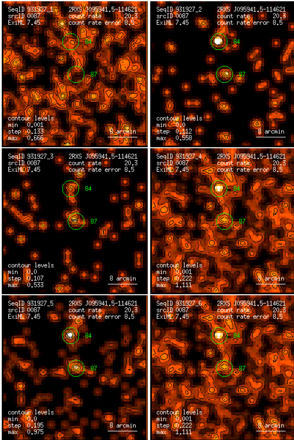
Figure 87: RASS 931927: detection 0087: band rate images, Gaussian filter: (1) PSPC channels 11 – 41, (2) 52 – 90, (3) 91 – 201, (4) 11 – 235, (5) 52 – 201, (6) 11 – 201. Broad band rates in counts/ks. Band rate contour levels in counts/ks/arcmin 2 .
