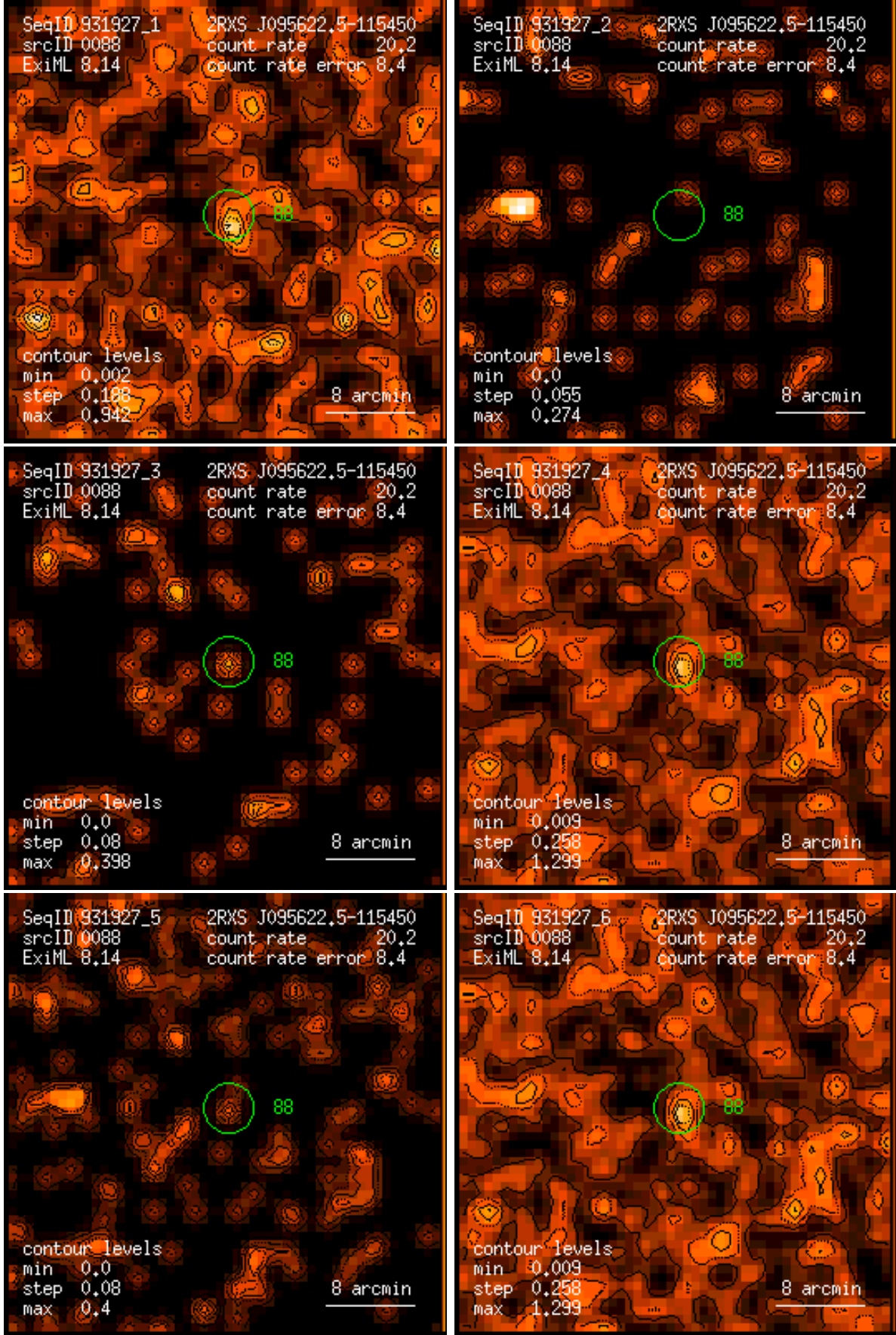
Figure 88: RASS 931927: detection 0088: band rate images, Gaussian filter: (1) PSPC channels 11 – 41, (2) 52 – 90, (3) 91 – 201, (4) 11 – 235, (5) 52 – 201, (6) 11 – 201. Broad band rates in counts/ks. Band rate contour levels in counts/ks/arcmin 2 .
