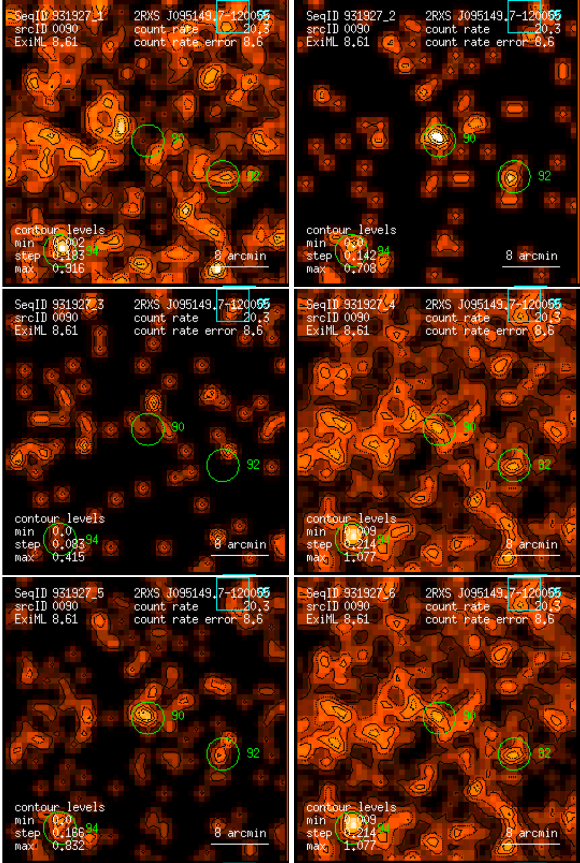
Figure 90: RASS 931927: detection 0090: band rate images, Gaussian filter: (1) PSPC channels 11 – 41, (2) 52 – 90, (3) 91 – 201, (4) 11 – 235, (5) 52 – 201, (6) 11 – 201. Broad band rates in counts/ks. Band rate contour levels in counts/ks/arcmin 2 .
