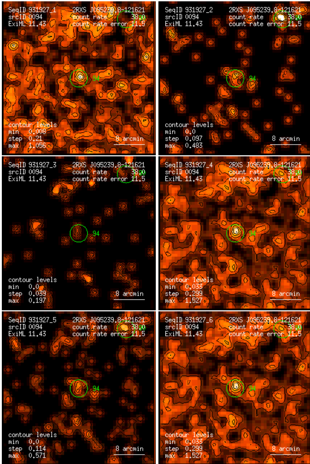
Figure 94: RASS 931927: detection 0094: band rate images, Gaussian filter: (1) PSPC channels 11 – 41, (2) 52 – 90, (3) 91 – 201, (4) 11 – 235, (5) 52 – 201, (6) 11 – 201. Broad band rates in counts/ks. Band rate contour levels in counts/ks/arcmin 2 .
