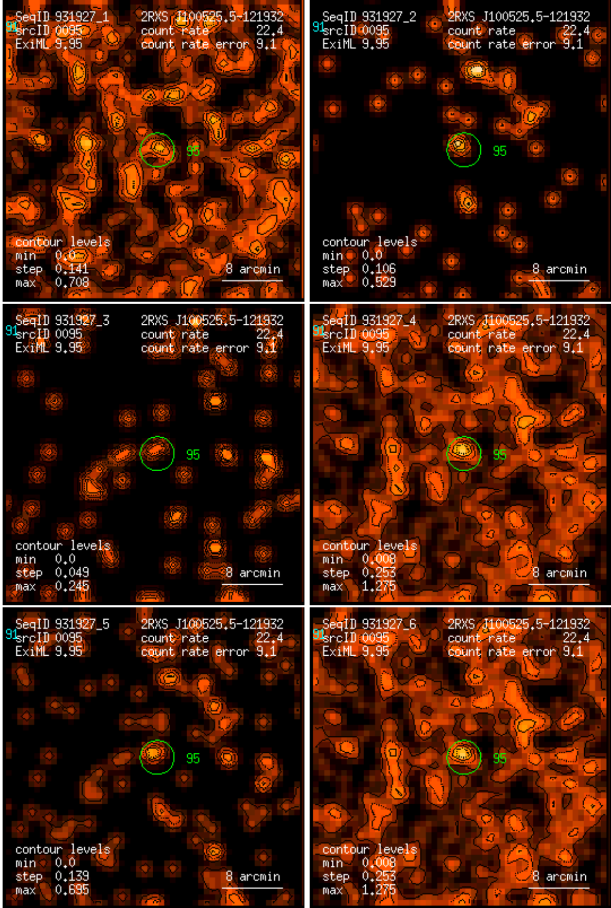
Figure 95: RASS 931927: detection 0095: band rate images, Gaussian filter: (1) PSPC channels 11 – 41, (2) 52 – 90, (3) 91 – 201, (4) 11 – 235, (5) 52 – 201, (6) 11 – 201. Broad band rates in counts/ks. Band rate contour levels in counts/ks/arcmin 2 .
