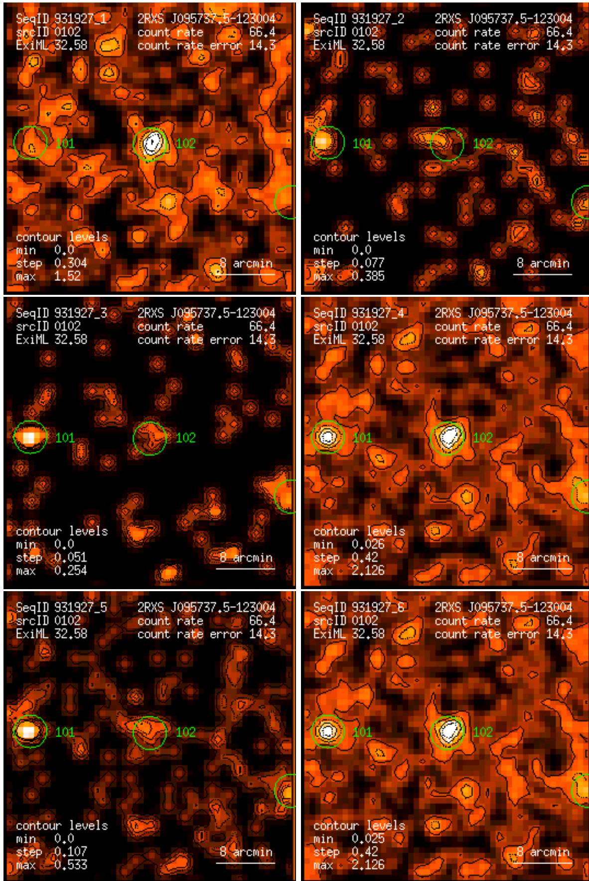
Figure 102: RASS 931927: detection 0102: band rate images, Gaussian filter: (1) PSPC channels 11 – 41, (2) 52 – 90, (3) 91 – 201, (4) 11 – 235, (5) 52 – 201, (6) 11 – 201. Broad band rates in counts/ks. Band rate contour levels in counts/ks/arcmin 2 .
