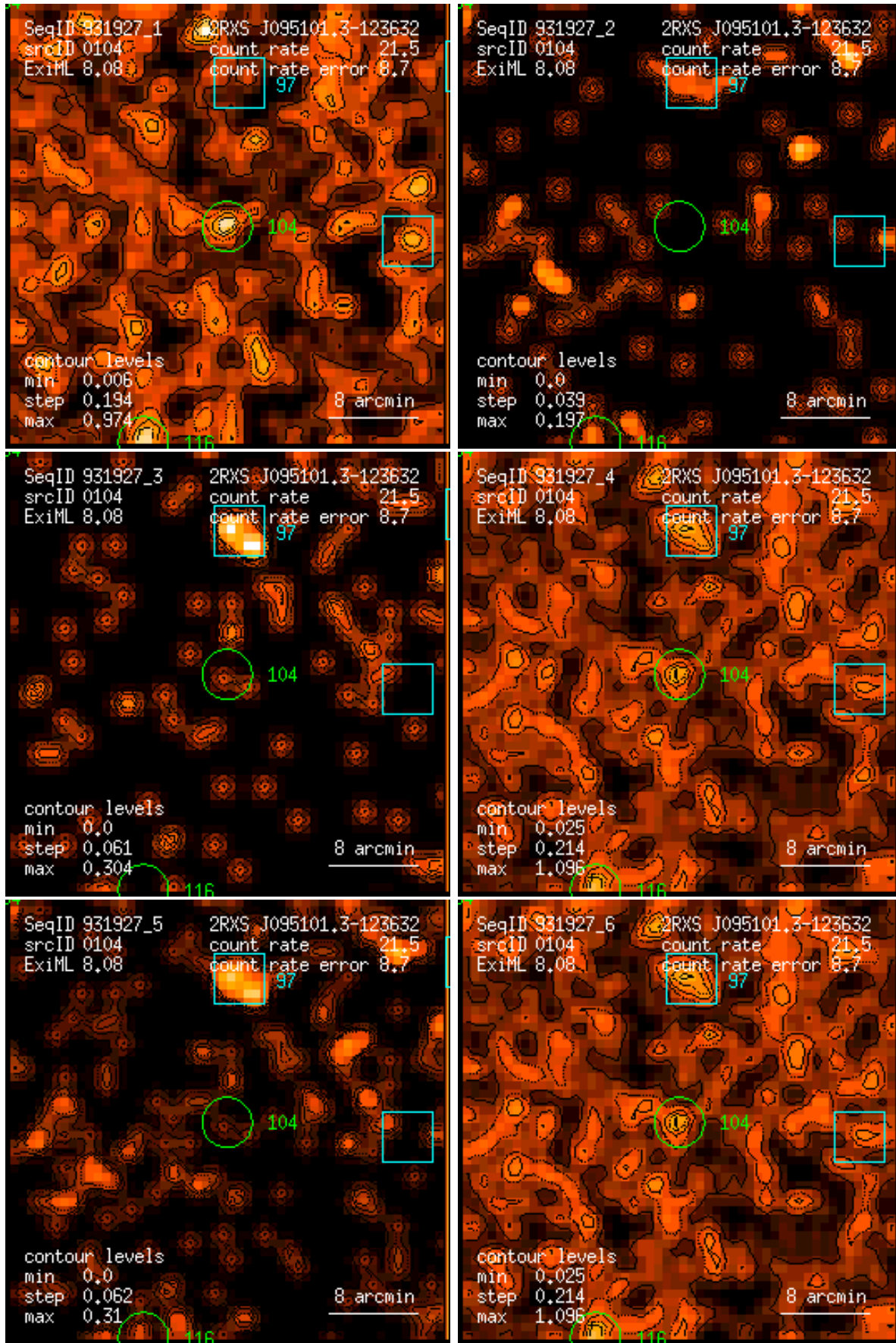
Figure 104: RASS 931927: detection 0104: band rate images, Gaussian filter: (1) PSPC channels 11 – 41, (2) 52 – 90, (3) 91 – 201, (4) 11 – 235, (5) 52 – 201, (6) 11 – 201. Broad band rates in counts/ks. Band rate contour levels in counts/ks/arcmin 2 .
