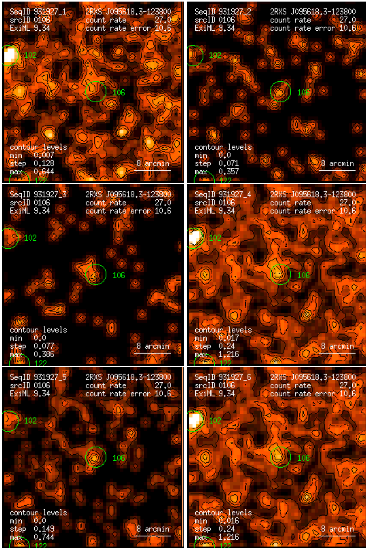
Figure 106: RASS 931927: detection 0106: band rate images, Gaussian filter: (1) PSPC channels 11 – 41, (2) 52 – 90, (3) 91 – 201, (4) 11 – 235, (5) 52 – 201, (6) 11 – 201. Broad band rates in counts/ks. Band rate contour levels in counts/ks/arcmin 2 .
