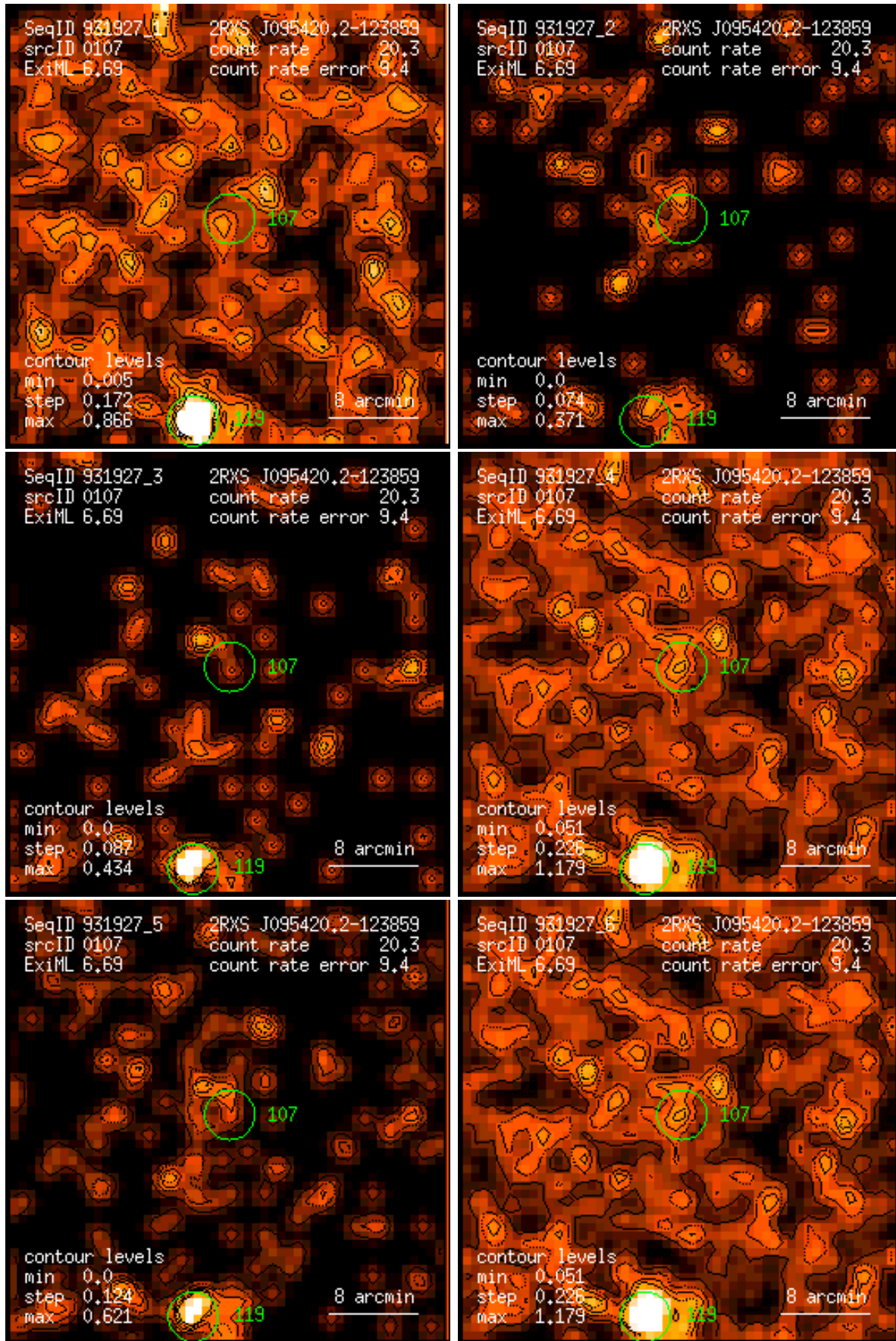
Figure 107: RASS 931927: detection 0107: band rate images, Gaussian filter: (1) PSPC channels 11 – 41, (2) 52 – 90, (3) 91 – 201, (4) 11 – 235, (5) 52 – 201, (6) 11 – 201. Broad band rates in counts/ks. Band rate contour levels in counts/ks/arcmin 2 .
