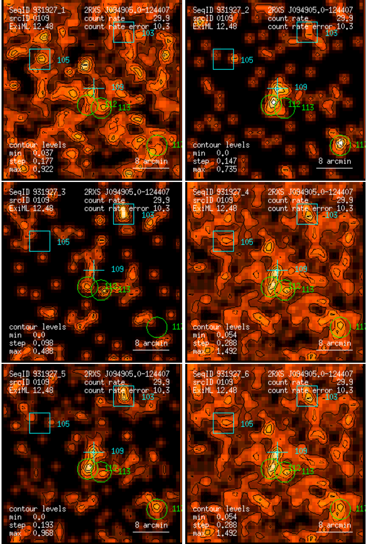
Figure 109: RASS 931927: detection 0109: band rate images, Gaussian filter: (1) PSPC channels 11 – 41, (2) 52 – 90, (3) 91 – 201, (4) 11 – 235, (5) 52 – 201, (6) 11 – 201. Broad band rates in counts/ks. Band rate contour levels in counts/ks/arcmin 2 .
