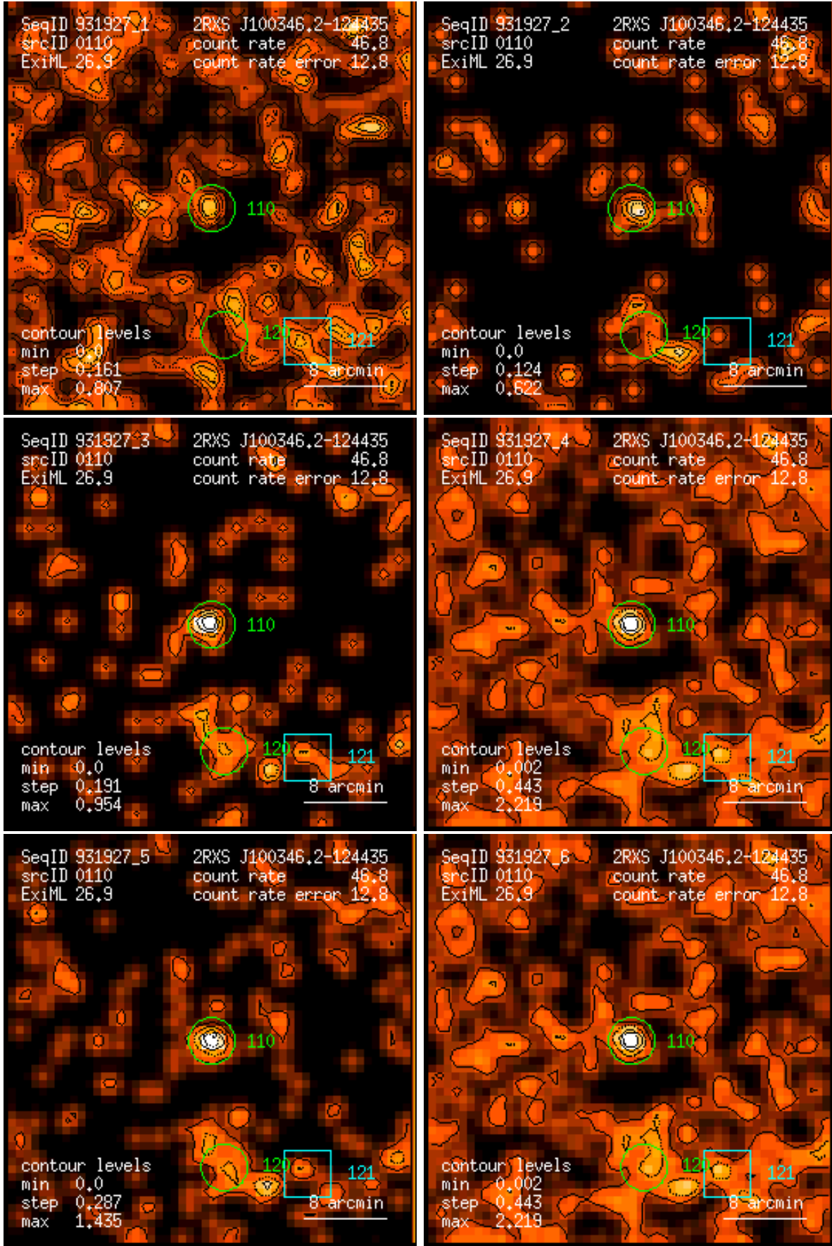
Figure 110: RASS 931927: detection 0110: band rate images, Gaussian filter: (1) PSPC channels 11 – 41, (2) 52 – 90, (3) 91 – 201, (4) 11 – 235, (5) 52 – 201, (6) 11 – 201. Broad band rates in counts/ks. Band rate contour levels in counts/ks/arcmin 2 .
