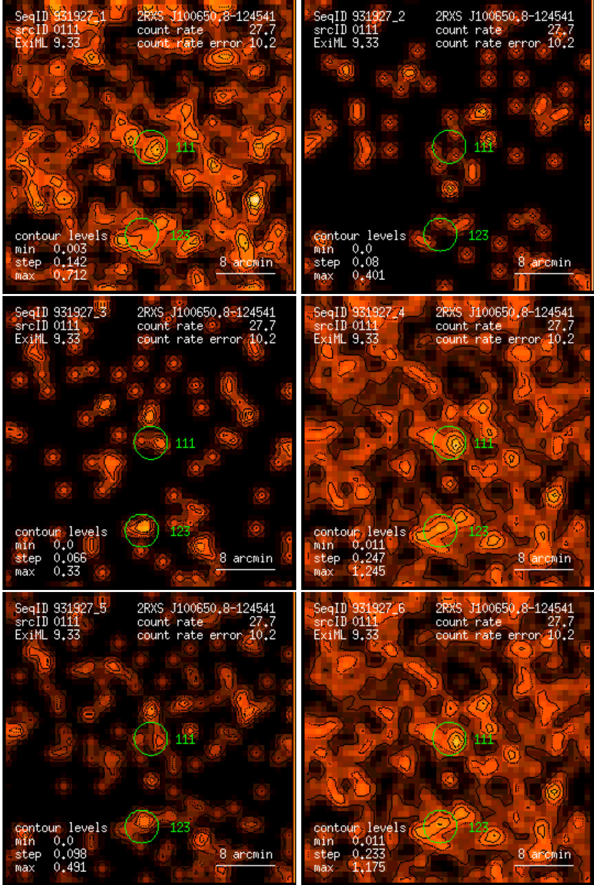
Figure 111: RASS 931927: detection 0111: band rate images, Gaussian filter: (1) PSPC channels 11 – 41, (2) 52 – 90, (3) 91 – 201, (4) 11 – 235, (5) 52 – 201, (6) 11 – 201. Broad band rates in counts/ks. Band rate contour levels in counts/ks/arcmin 2 .
