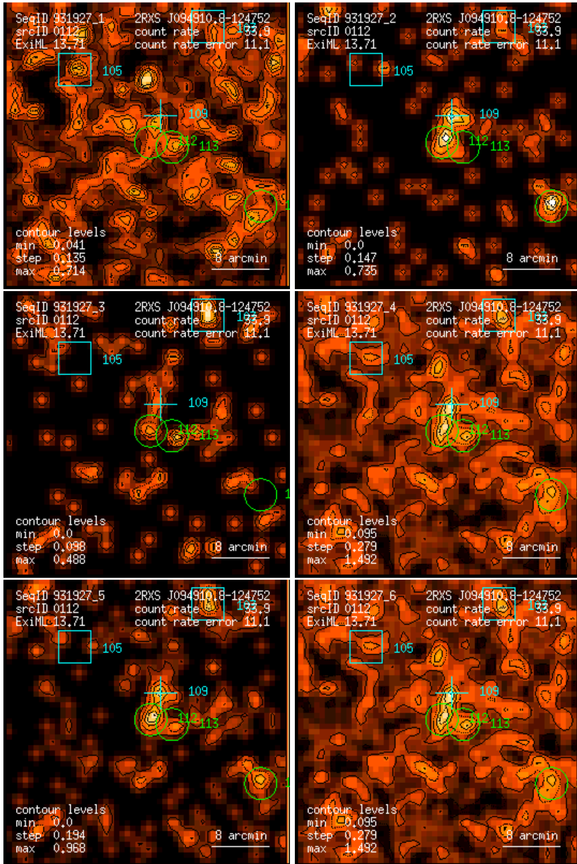
Figure 112: RASS 931927: detection 0112: band rate images, Gaussian filter: (1) PSPC channels 11 – 41, (2) 52 – 90, (3) 91 – 201, (4) 11 – 235, (5) 52 – 201, (6) 11 – 201. Broad band rates in counts/ks. Band rate contour levels in counts/ks/arcmin 2 .
